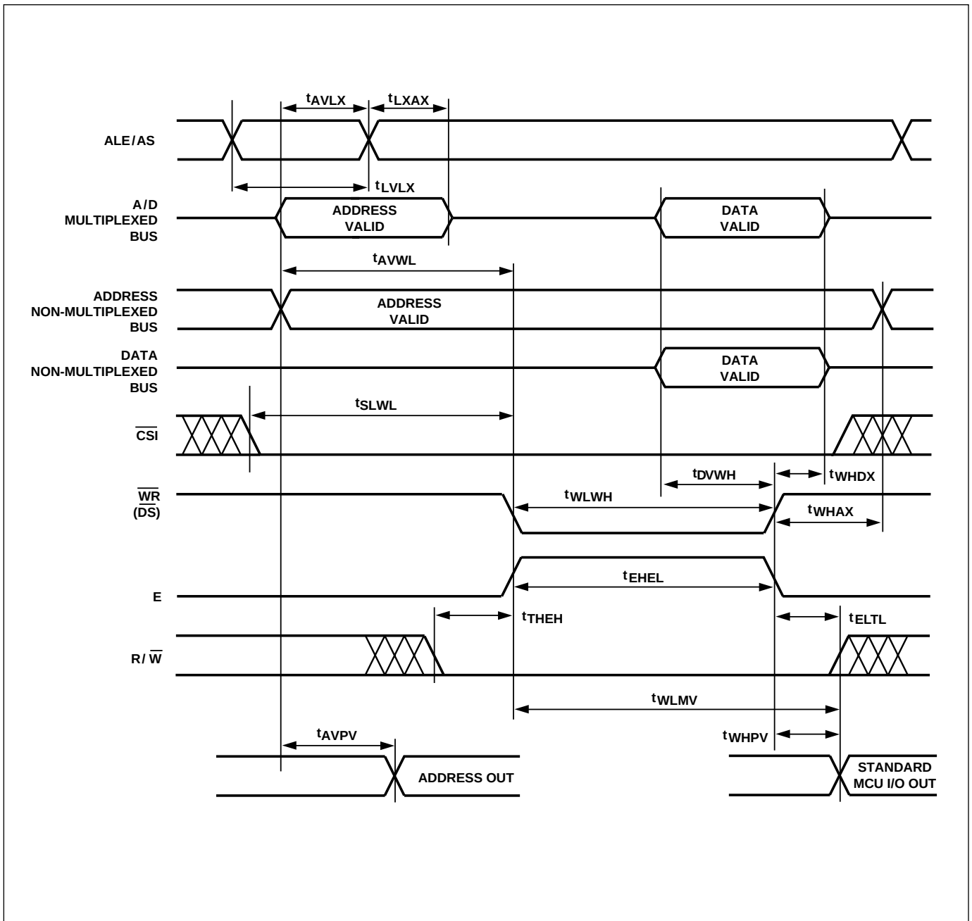
Figure 30. Write Timing
