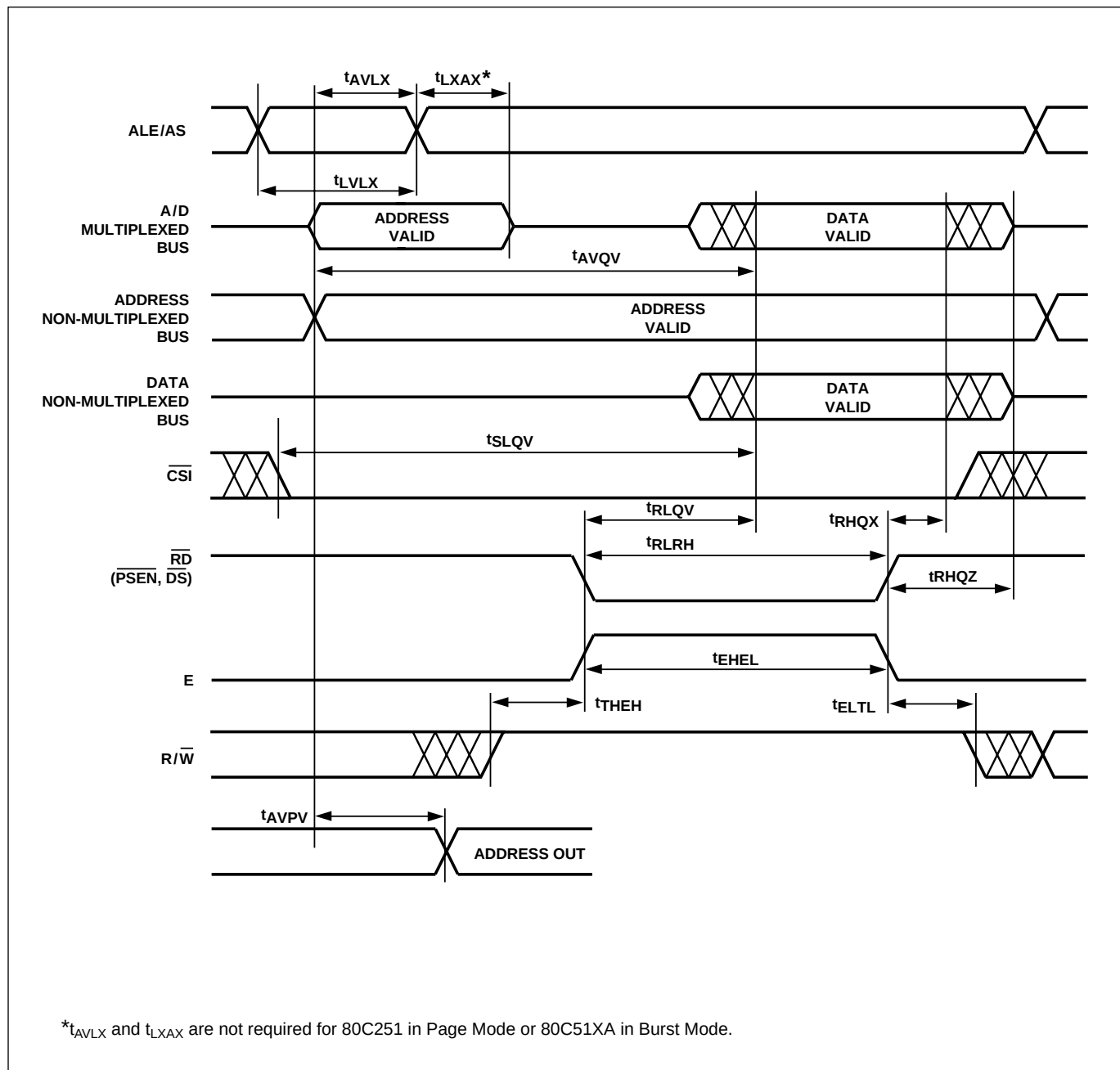
Figure 29. Read Timing
