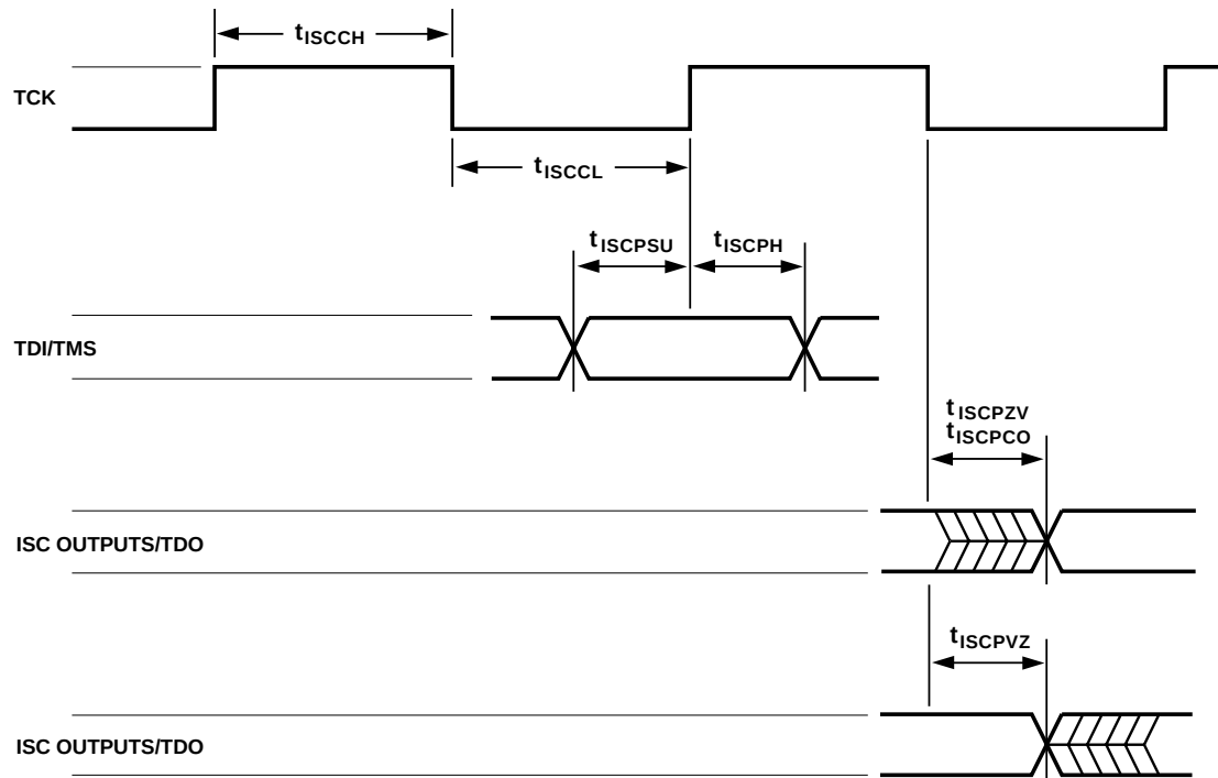
Figure 32. ISC Timing
