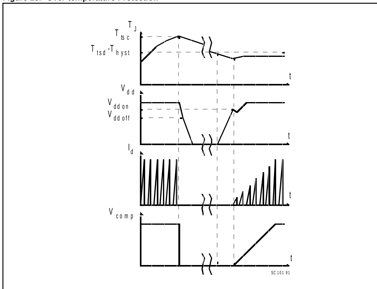
Figure 13. Over-temperature Protection
