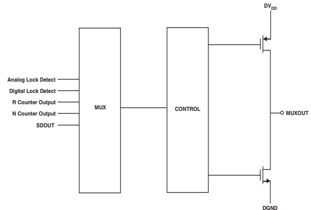
Figure 6. MUXOUT Circuit
