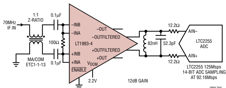
ADC Driver with Single-Ended to Differential Conversion
