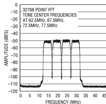
4-Tone WCDMA Waveform, LT1993-4 Driving LTC2255 14-Bit ADC at 92.16Msps
