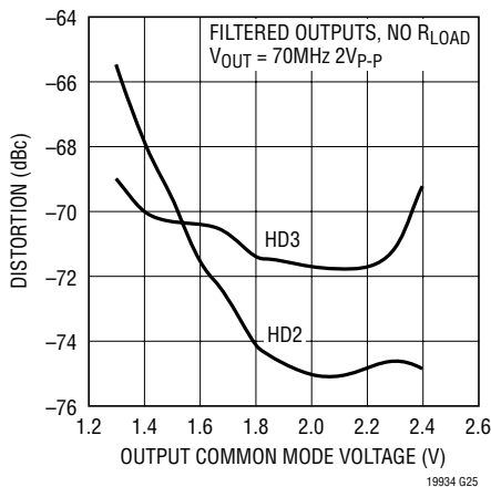
Distortion vs Output Common Mode Voltage, LT1993-4 Driving LTC2249 14-Bit ADC
