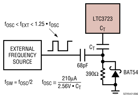
Figure 5. Synchronization from External Source
