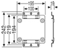
Dimension drawing
