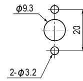
取付穴図 Hole for Installation
