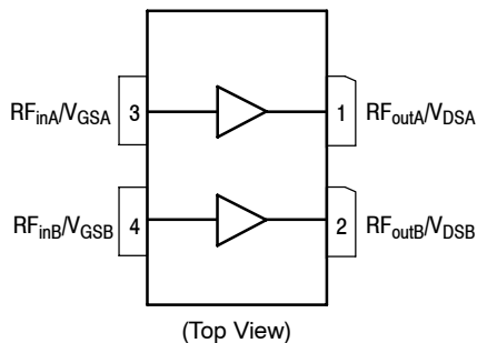
Figure 1. Pin Connections
