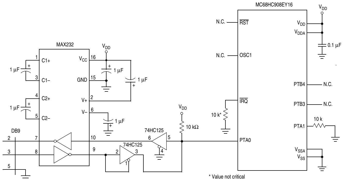
Figure 19-11. Forced Monitor Mode ( \overline{\text{IRQ}} = V_{SS} )
