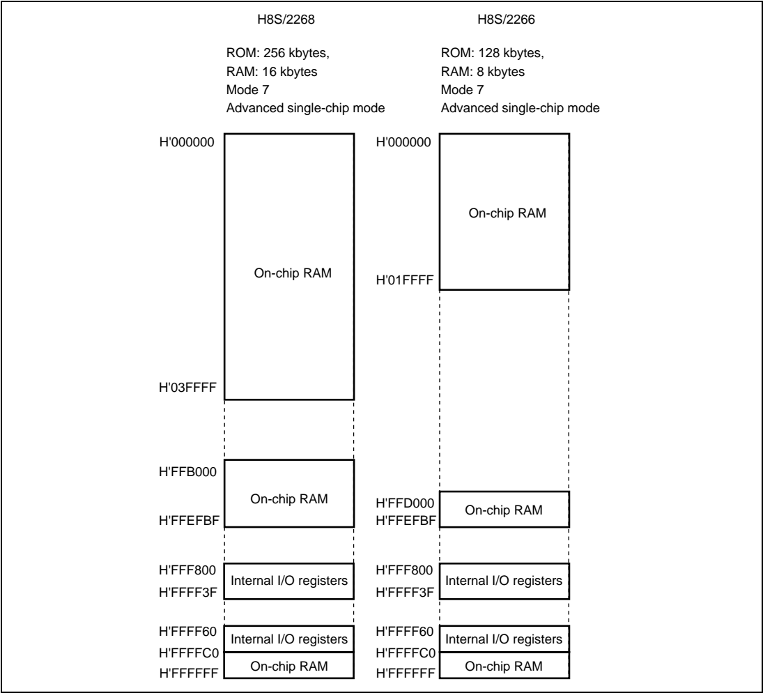
Figure 3.1 Address Map (1)
