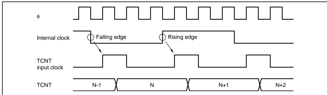
Figure 10.31 Count Timing in Internal Clock Operation
