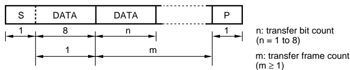
Figure 14.4 I 2 C Bus Data Format (Serial Format)
