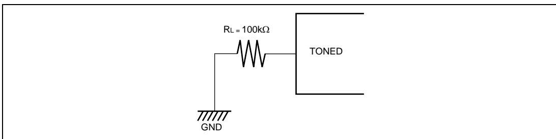
Figure 25.12 TONED Load Circuit (Supported only by the H8S/2268 Group)
