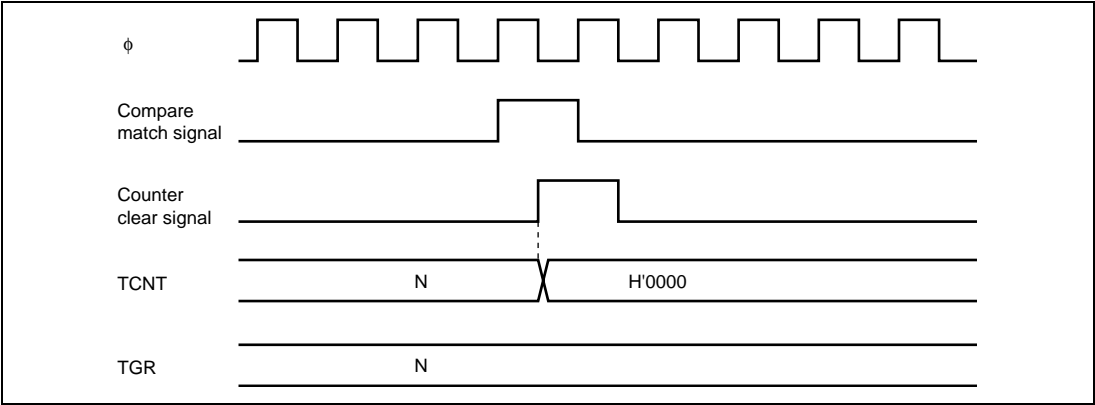
Figure 10.35 Counter Clear Timing (Compare Match)
