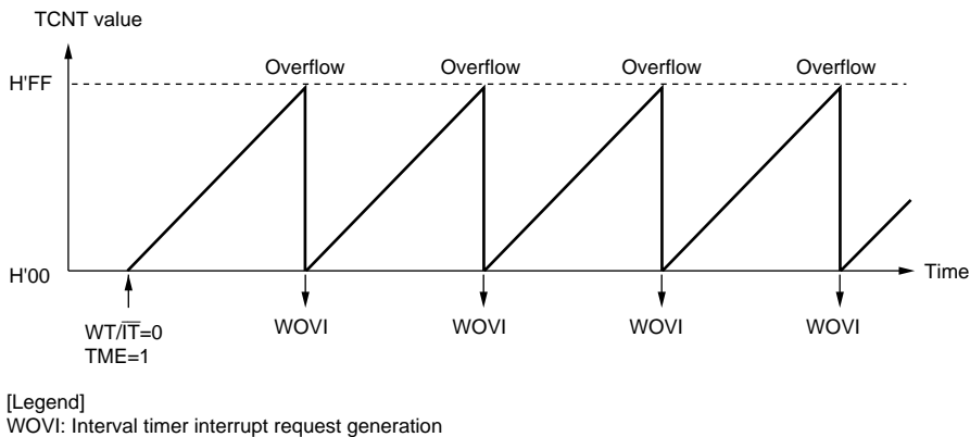
Figure 12.4 Interval Timer Mode Operation
