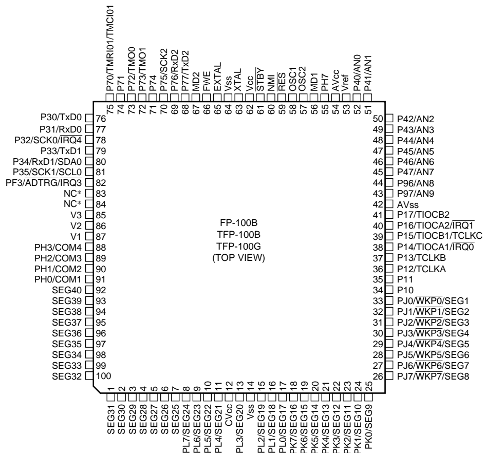
Figure 1.4 Pin Arrangement of H8S/2264 Group
