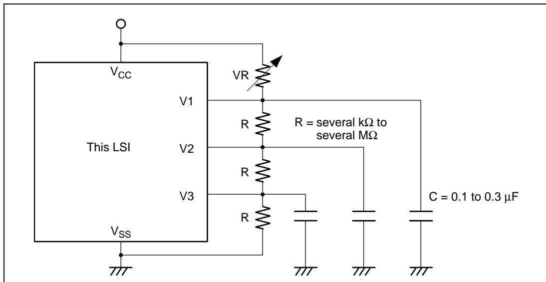
Figure 17.12 Connection of External Split-Resistance
