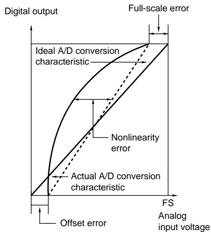
Figure 15.7 A/D Conversion Accuracy Definitions (2)
