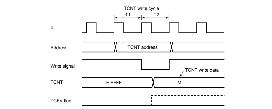
Figure 10.54 Contention between TCNT Write and Overflow
