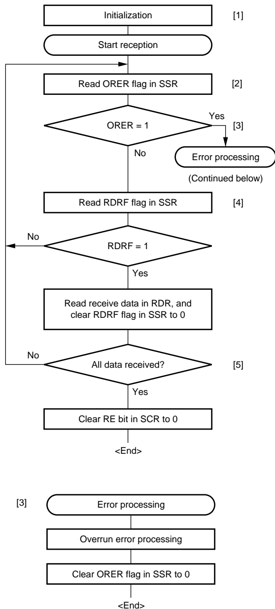
Figure 13.22 Sample Serial Reception Flowchart
