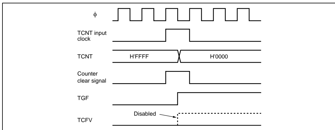
Figure 10.53 Contention between Overflow and Counter Clearing
