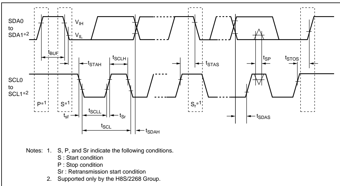
Figure 25.11 I²C Bus Interface Input/Output Timing (Option)
