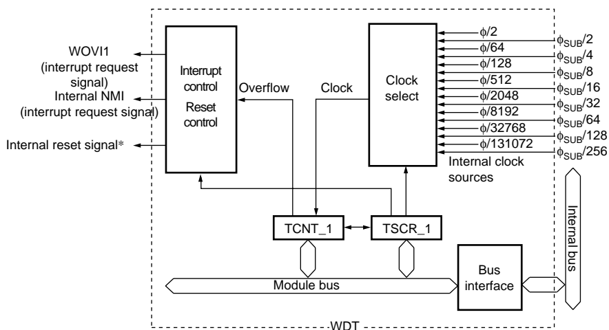
Figure 12.1 Block Diagram of WDT_0
