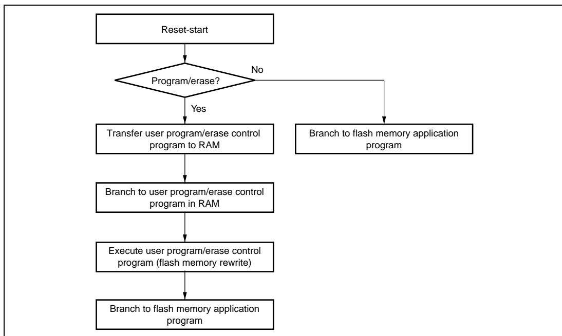
Figure 20.7 Programming/Erasing Flowchart Example in User Program Mode
