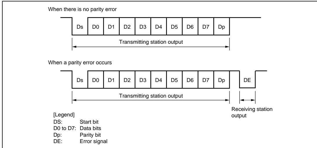
Figure 13.25 Normal Smart Card Interface Data Format
