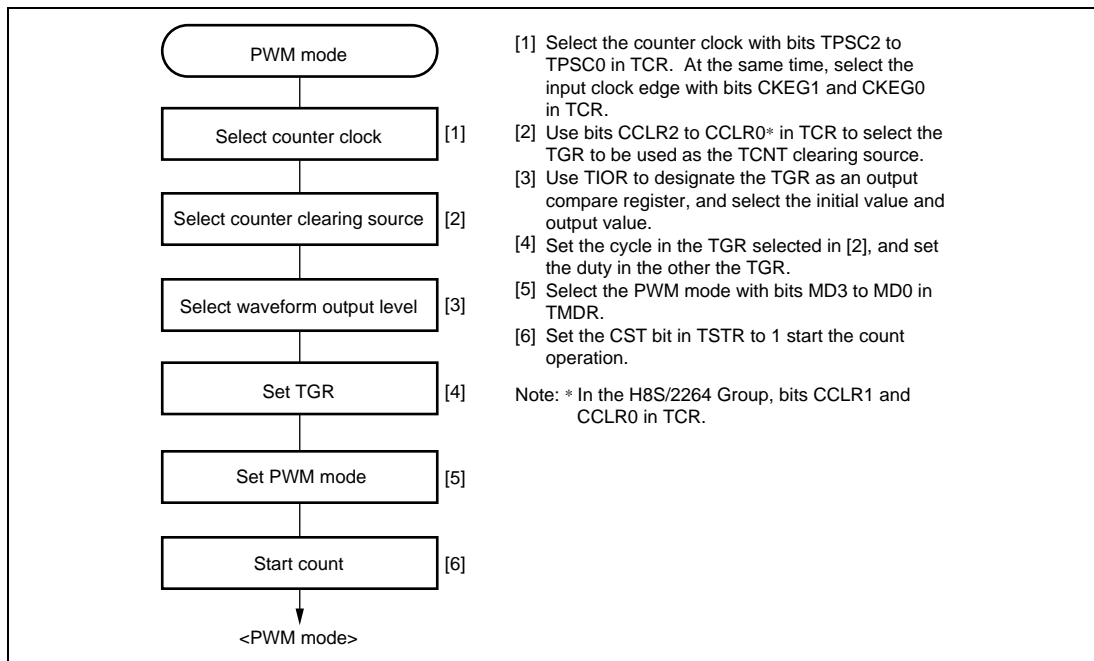
Figure 10.22 Example of PWM Mode Setting Procedure
