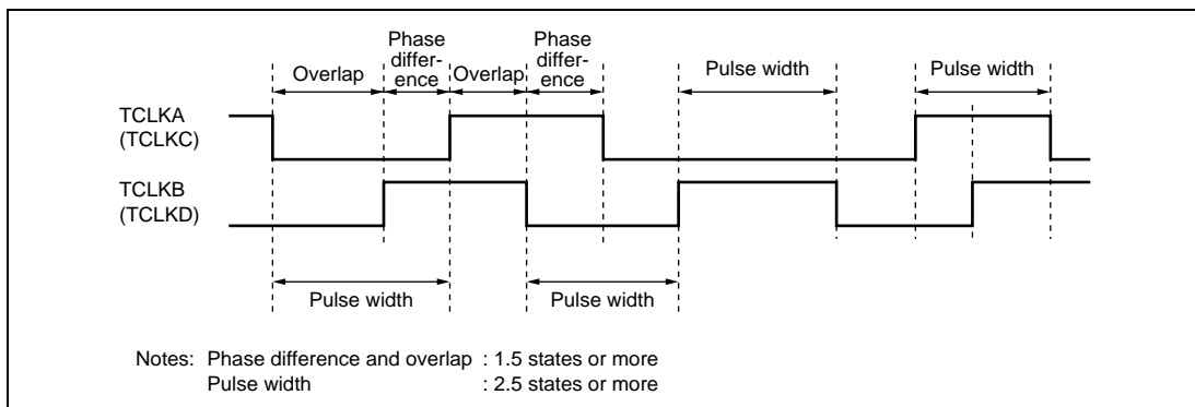
Figure 10.45 Phase Difference, Overlap, and Pulse Width in Phase Counting Mode (H8S/2268 Group Only)
