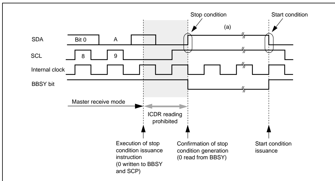
Figure 14.17 Points for Attention Concerning Reading of Master Receive Data
