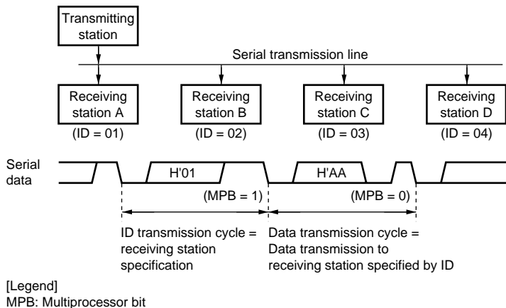
Figure 13.13 Example of Communication Using Multiprocessor Format (Transmission of Data H'AA to Receiving Station A)
