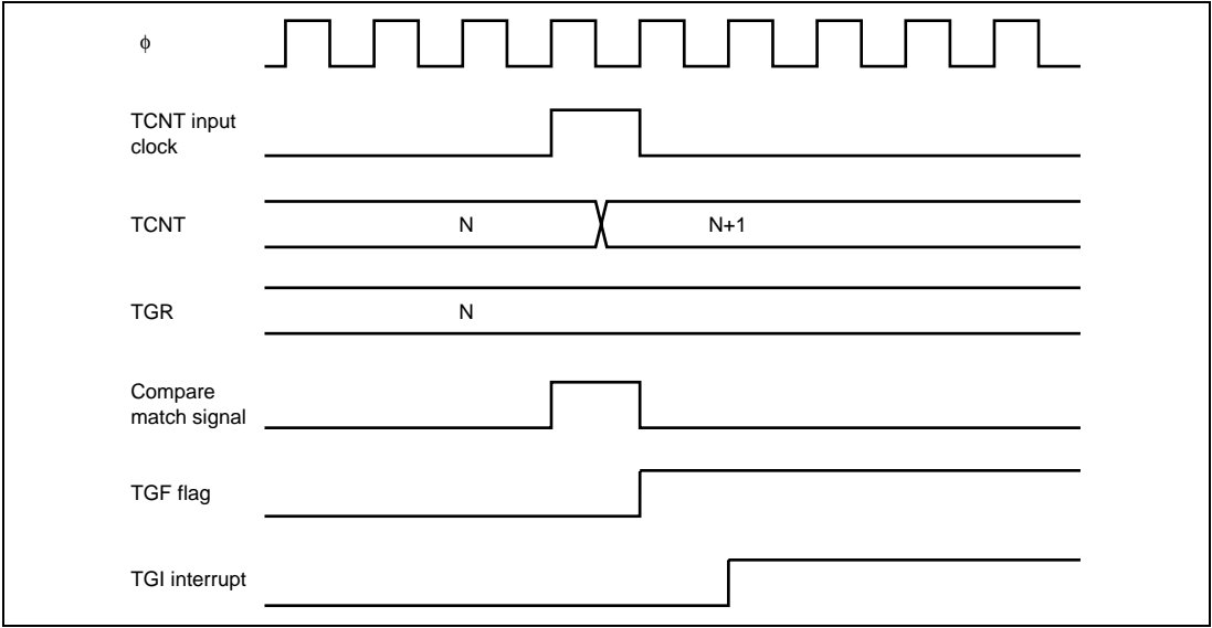
Figure 10.39 TGI Interrupt Timing (Compare Match)
