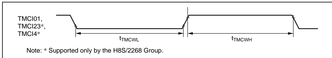
Figure 25.8 8-Bit Timer Clock Input Timing
