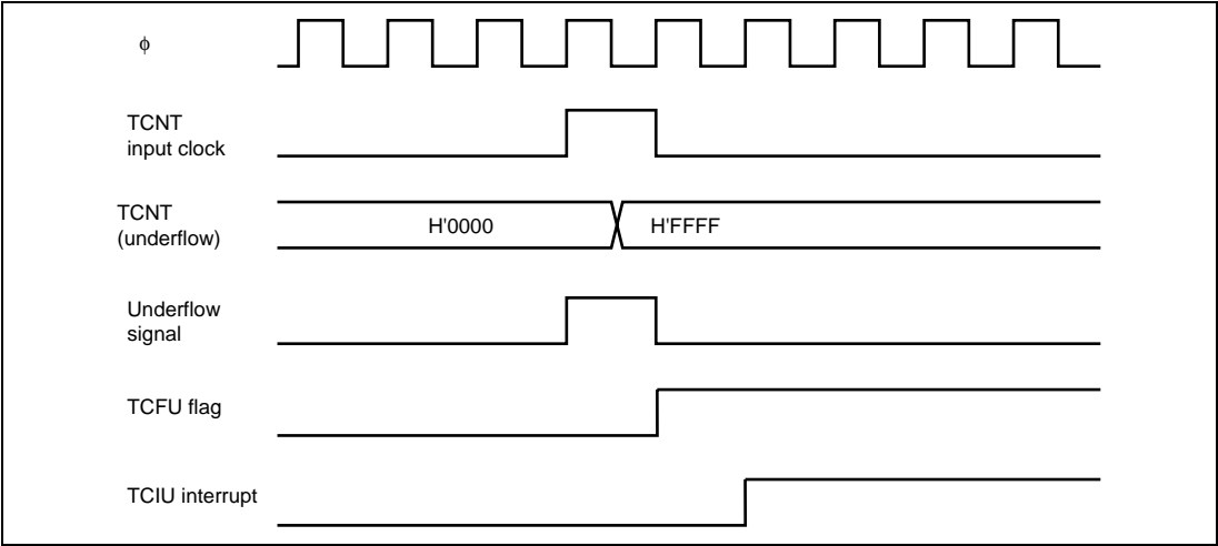
Figure 10.42 TCIU Interrupt Setting Timing (H8S/2268 Group Only)
