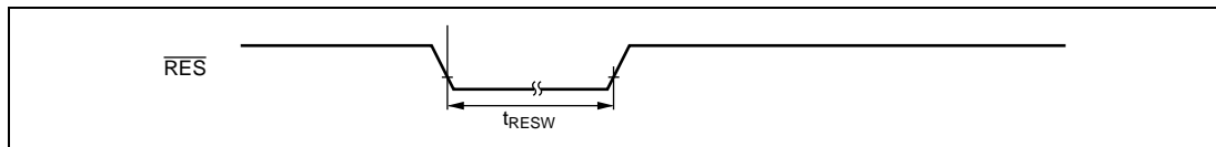
Figure 25.5 Reset Input Timing
