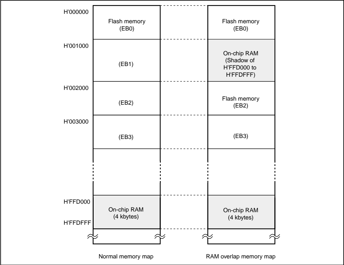
Figure 20.9 Example of RAM Overlap Operation
