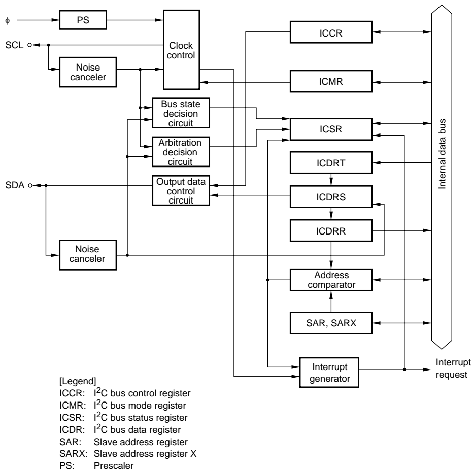
Figure 14.1 Block Diagram of I²C Bus Interface
