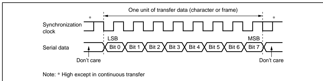
Figure 13.17 Data Format in Synchronous Communication (For LSB-First)
