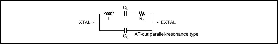
Figure 21.3 Crystal Resonator Equivalent Circuit
