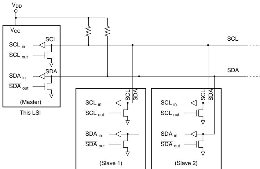
Figure 14.2 I 2 C Bus Interface Connections (Example: This LSI as Master)
