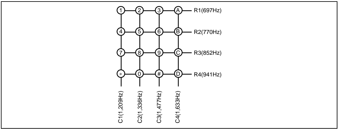
Figure 18.1 DTMF Frequencies
