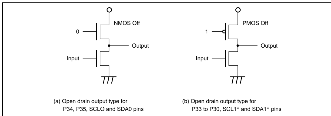
Figure 9.1 Types of Open Drain Outputs
