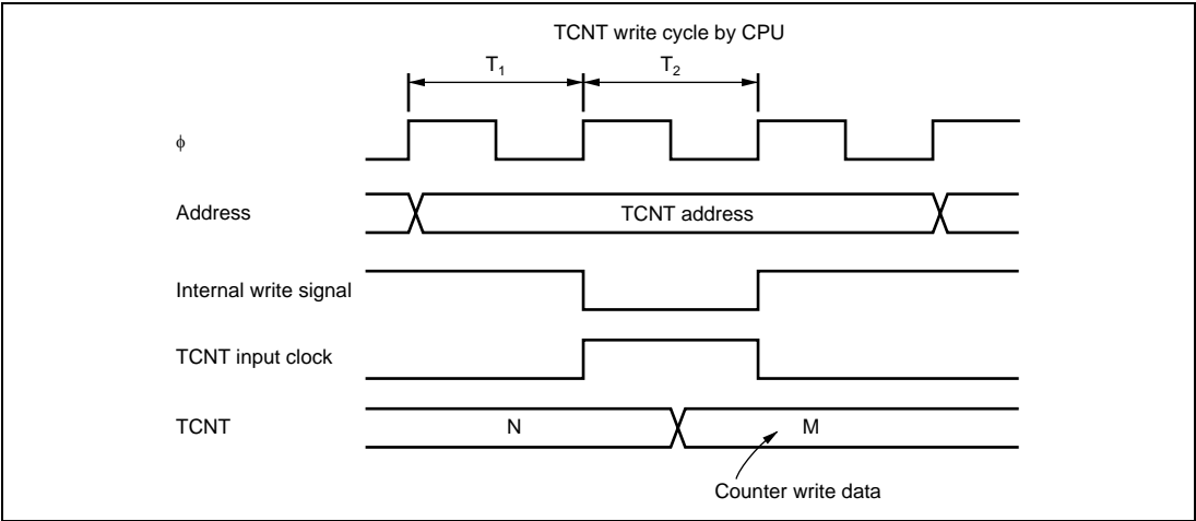
Figure 11.11 Contention between TCNT Write and Increment
