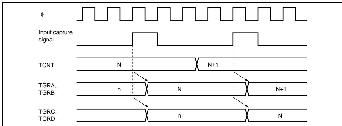
Figure 10.38 Buffer Operation Timing (Input Capture)
