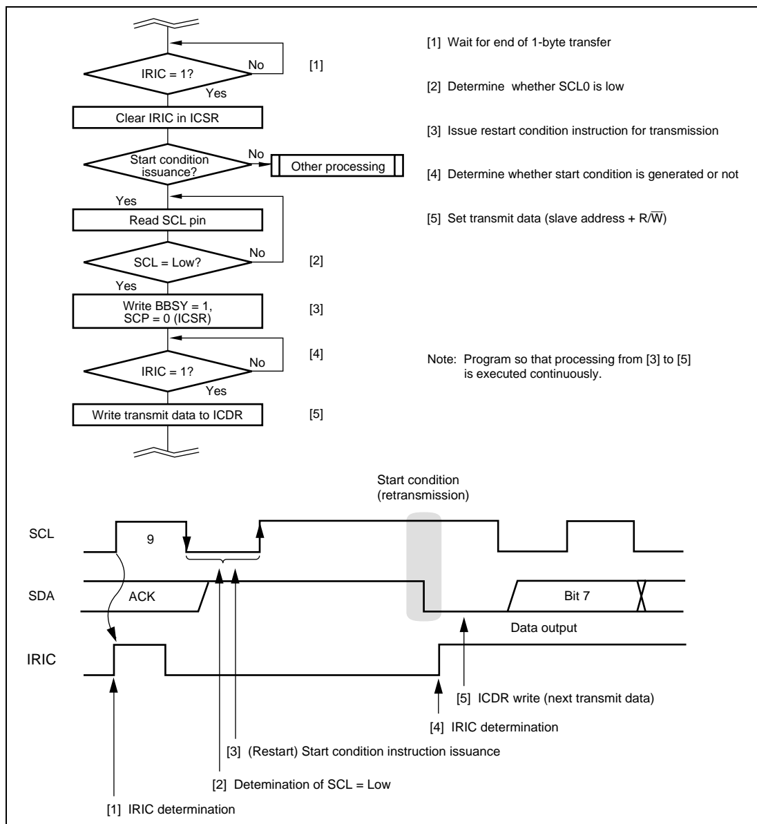
Figure 14.18 Flowchart and Timing of Start Condition Instruction Issuance for Retransmission
