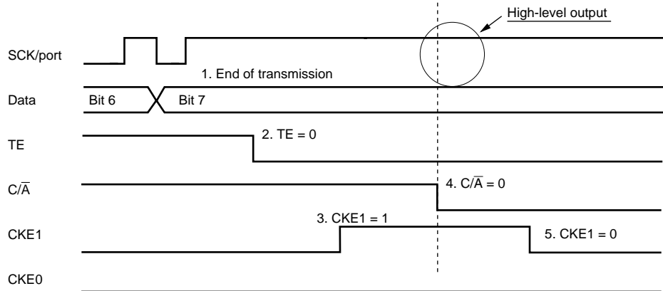
Figure 13.42 Operation when Switching from SCK Pin Function to Port Pin Function (Example of Preventing Low-Level Output)
