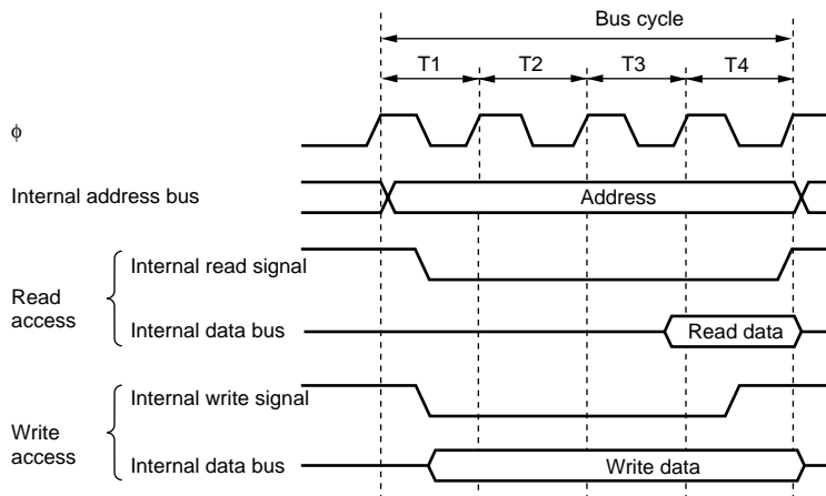
Figure 7.3 On-Chip Peripheral Module Access Cycle (H'FFFC30 to H'FFCA3)
