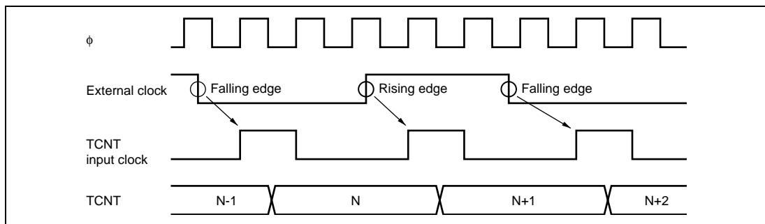
Figure 10.32 Count Timing in External Clock Operation
