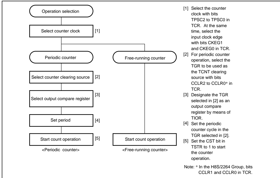
Figure 10.7 Example of Counter Operation Setting Procedure
