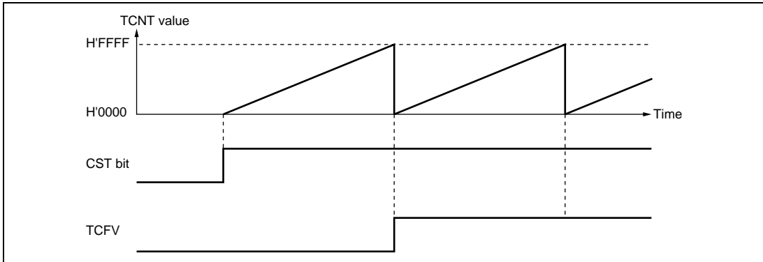
Figure 10.8 Free-Running Counter Operation
