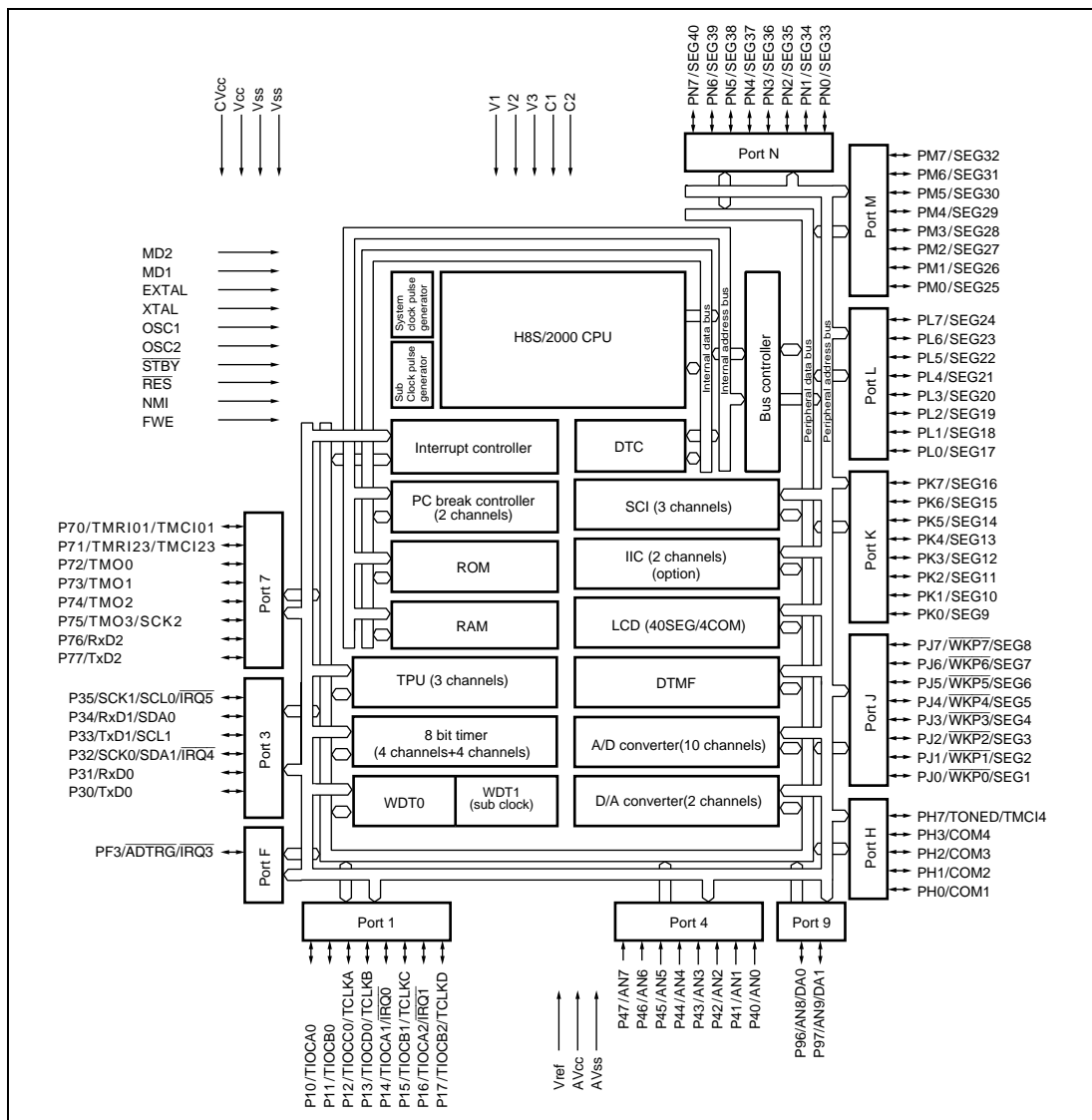
Figure 1.1 Internal Block Diagram of H8S/2268 Group
