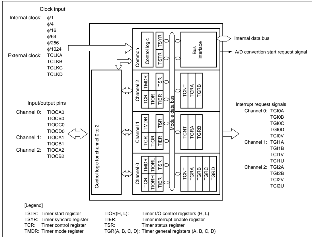
Figure 10.1 Block Diagram of TPU for H8S/2268 Group
