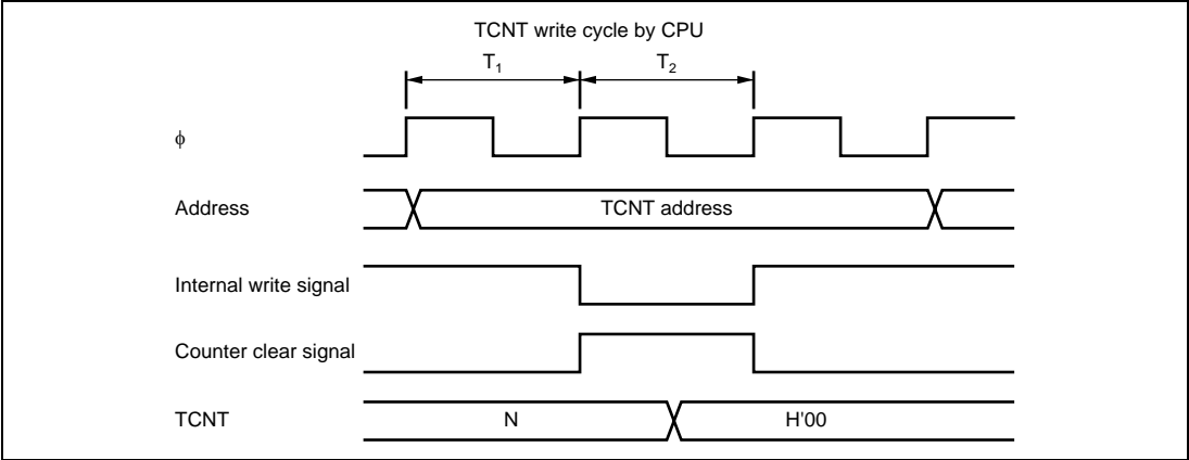
Figure 11.10 Contention between TCNT Write and Clear
