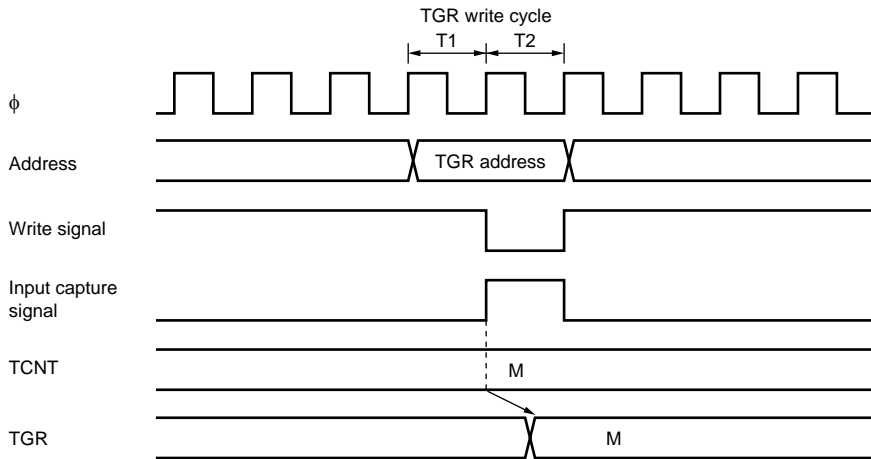
Figure 10.51 Contention between TGR Write and Input Capture
