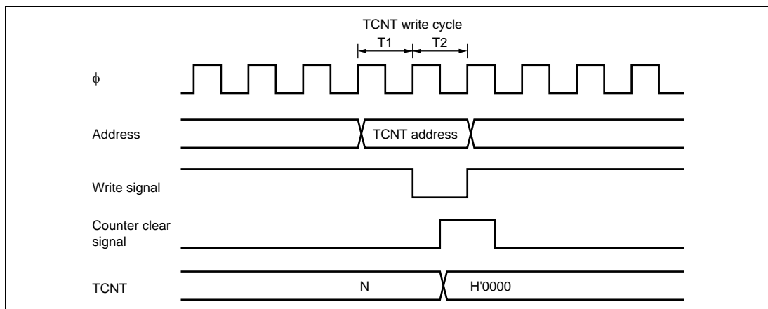
Figure 10.46 Contention between TCNT Write and Clear Operations
