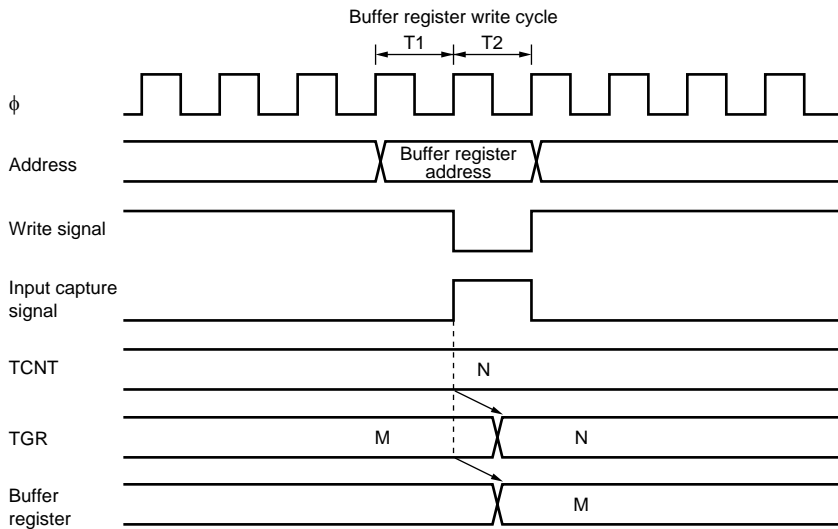
Figure 10.52 Contention between Buffer Register Write and Input Capture
