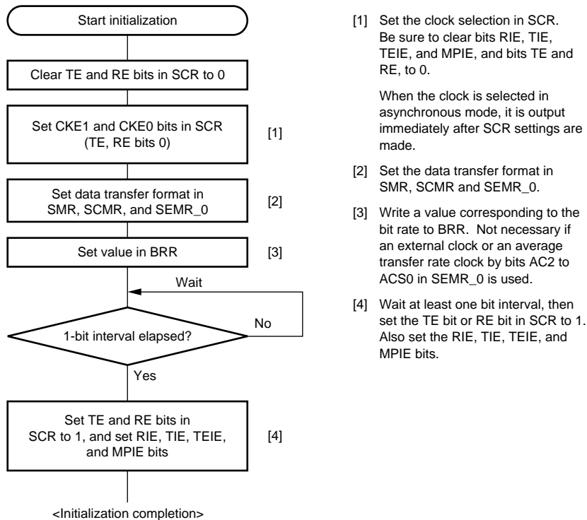
Figure 13.8 Sample SCI Initialization Flowchart
