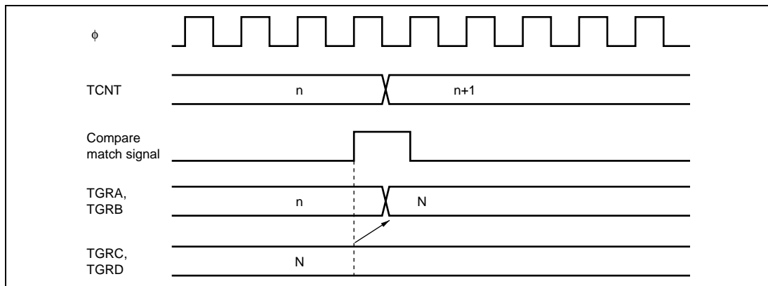
Figure 10.37 Buffer Operation Timing (Compare Match)
