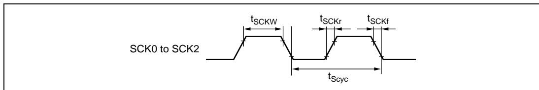
Figure 25.9 SCK Clock Input Timing
