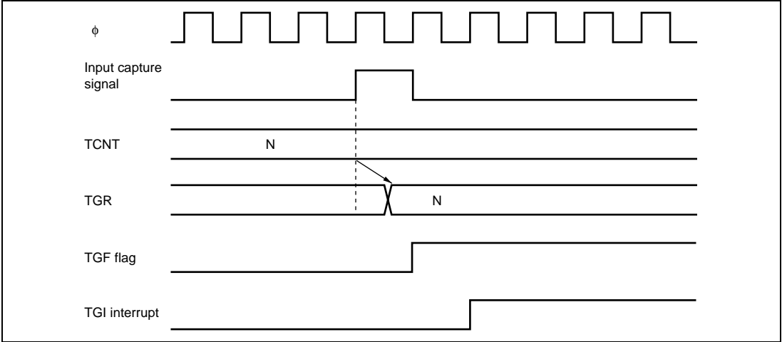
Figure 10.40 TGI Interrupt Timing (Input Capture)
