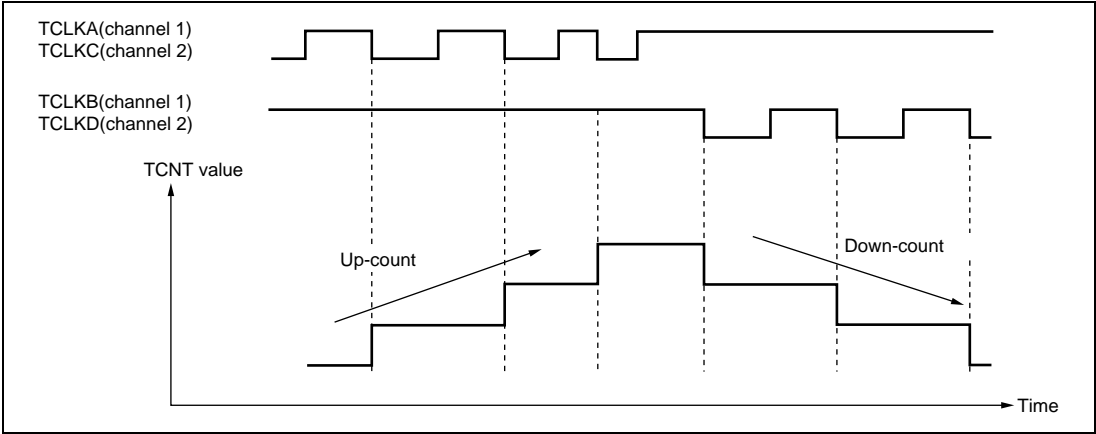
Figure 10.29 Example of Phase Counting Mode 3 Operation
