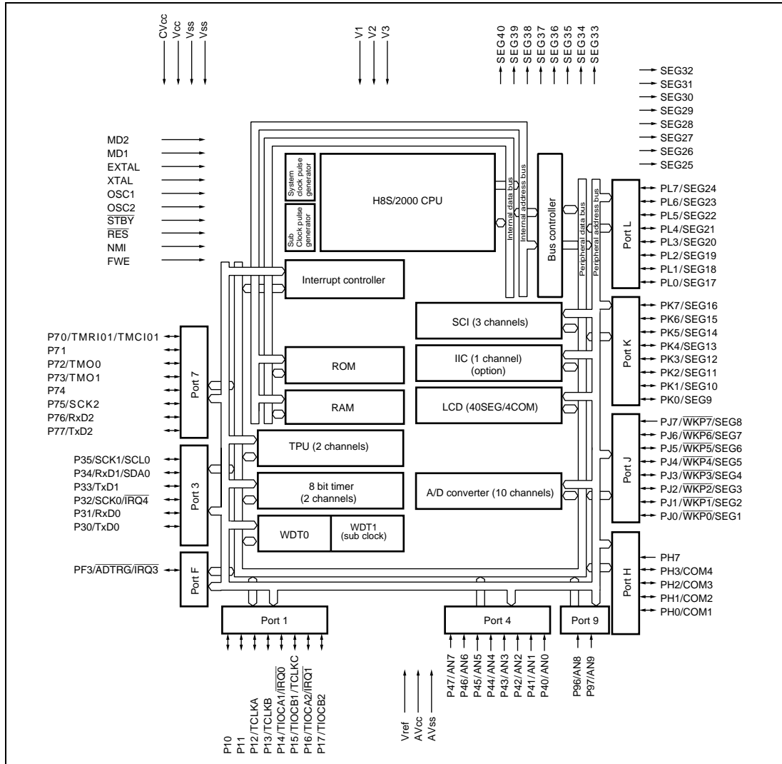
Figure 1.2 Internal Block Diagram of H8S/2264 Group
