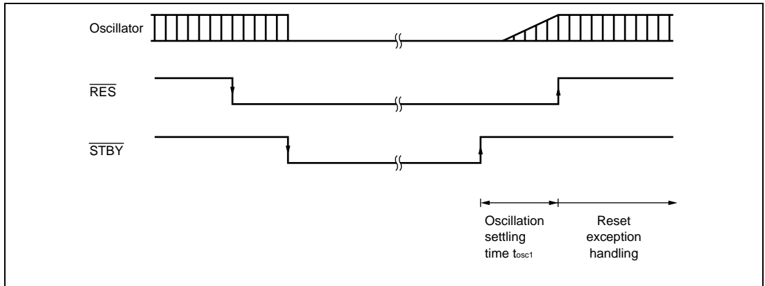
Figure 22.4 Hardware Standby Mode Timing
