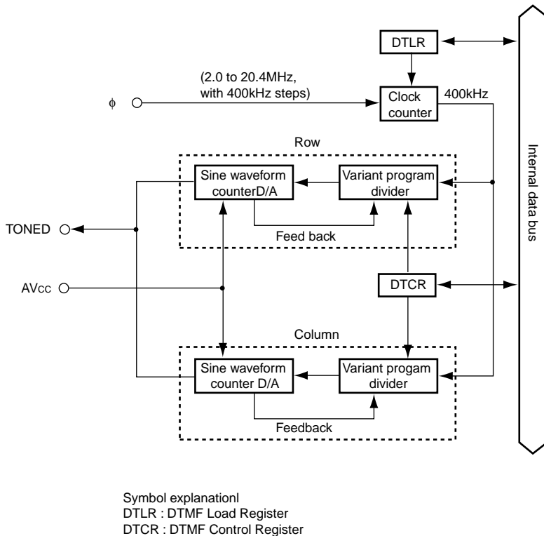
Figure 18.2 DTMF Generation Circuit Diagram
