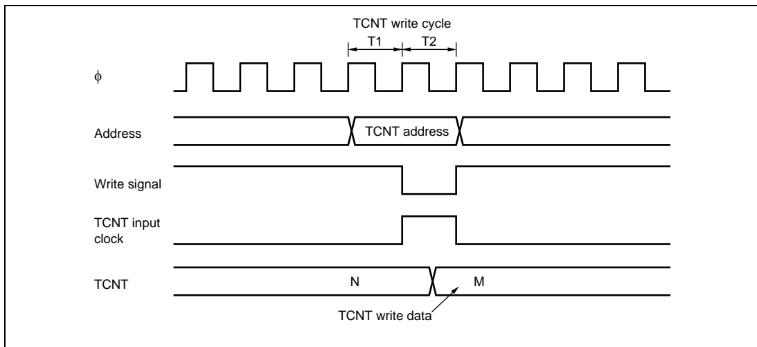
Figure 10.47 Contention between TCNT Write and Increment Operations
