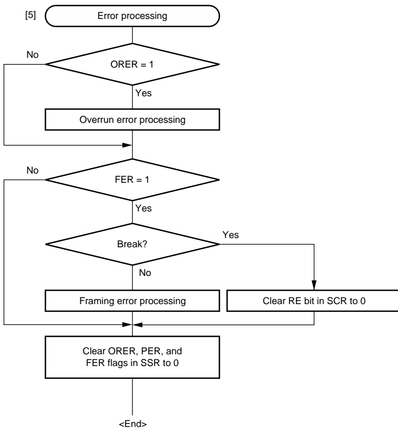
Figure 13.16 Sample Multiprocessor Serial Reception Flowchart (2)
