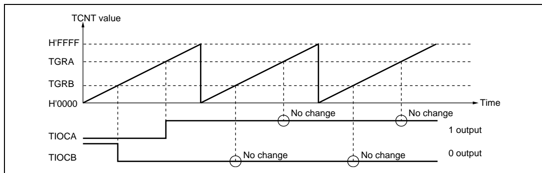
Figure 10.11 Example of 0 Output/1 Output Operation
