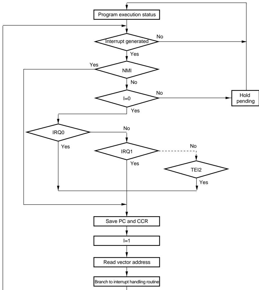
Figure 5.9 Flowchart of Procedure up to Interrupt Acceptance in Interrupt Control Mode 0
