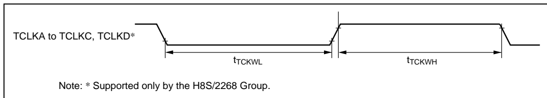
Figure 25.7 TPU Clock Input Timing
