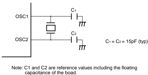
Figure 21.8 Example Connection of 32.768-kHz Crystal Resonator
