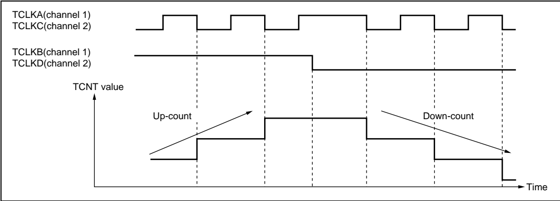
Figure 10.28 Example of Phase Counting Mode 2 Operation
