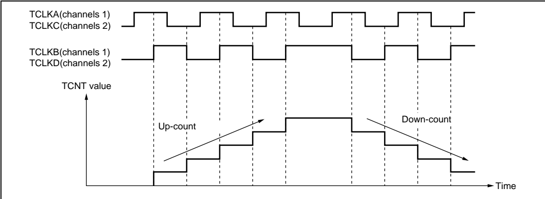
Figure 10.30 Example of Phase Counting Mode 4 Operation
