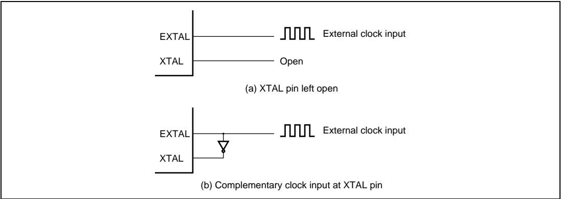
Figure 21.4 External Clock Input (Examples)
