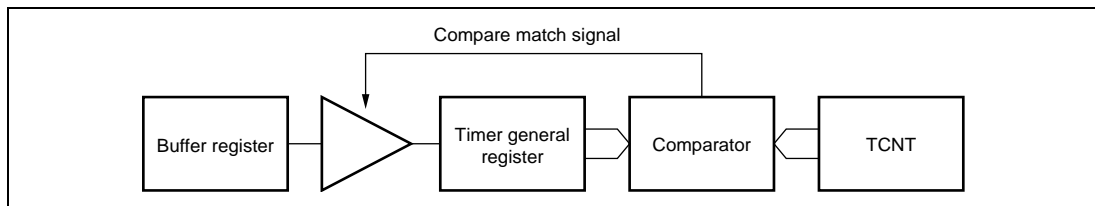
Figure 10.17 Compare Match Buffer Operation
