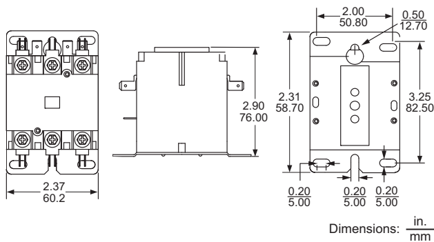
Figure 3: Type DPA, 2 and 3 Pole 20–40 Full Load Amperes
