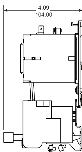
Figure 7: Approximate Dimensions
