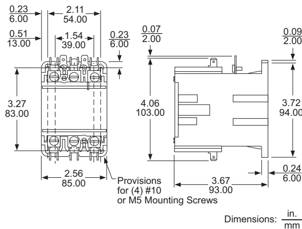
Figure 5: Type DPA, 2 and 3 Pole 50 and 60 Full Load Amperes
