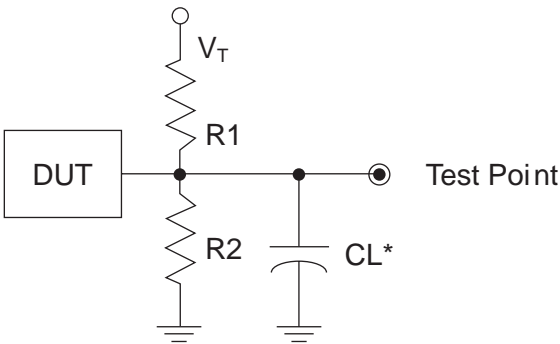
Figure 3-15. Output Test Load, LVTTTL and LVCMOS Standards
