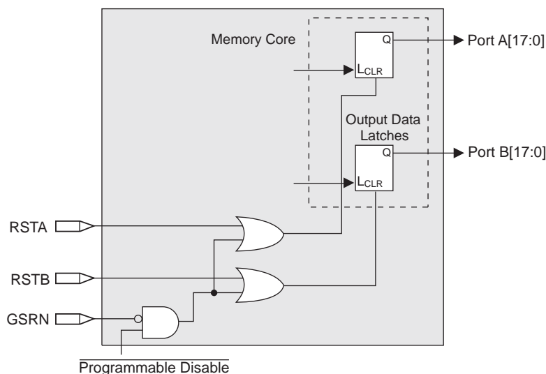
Figure 2-18. Memory Core Reset
