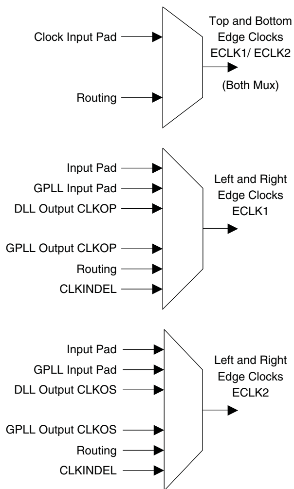
Figure 2-17. Edge Clock Mux Connections
