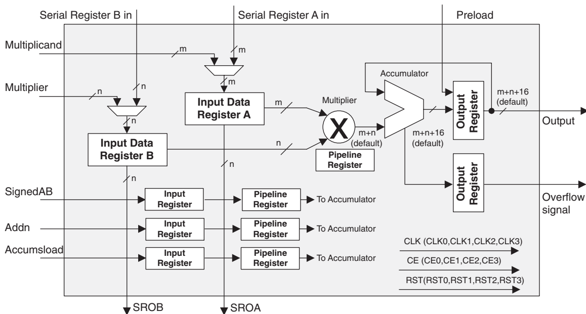
Figure 2-21. MAC sysDSP
