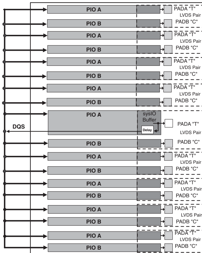
Figure 2-31. DQS Routing for the Bottom Edge of the Device
