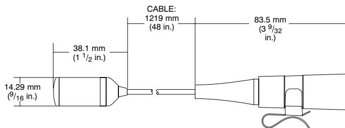
OVERALL DIMENSIONS FIGURE 2
