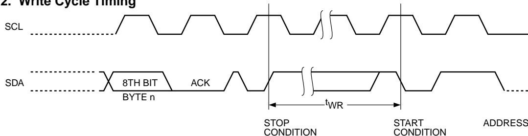
Figure 3. Start/Stop Timing
