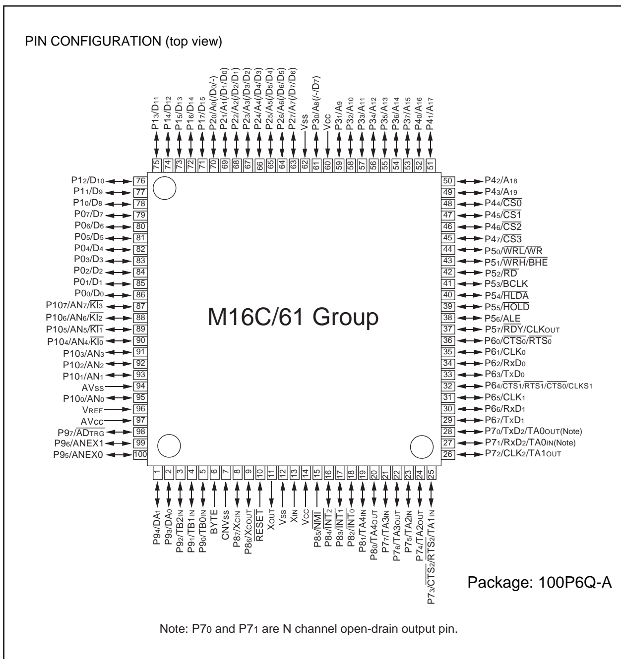
Figure 1.1.2. Pin configuration (top view)
