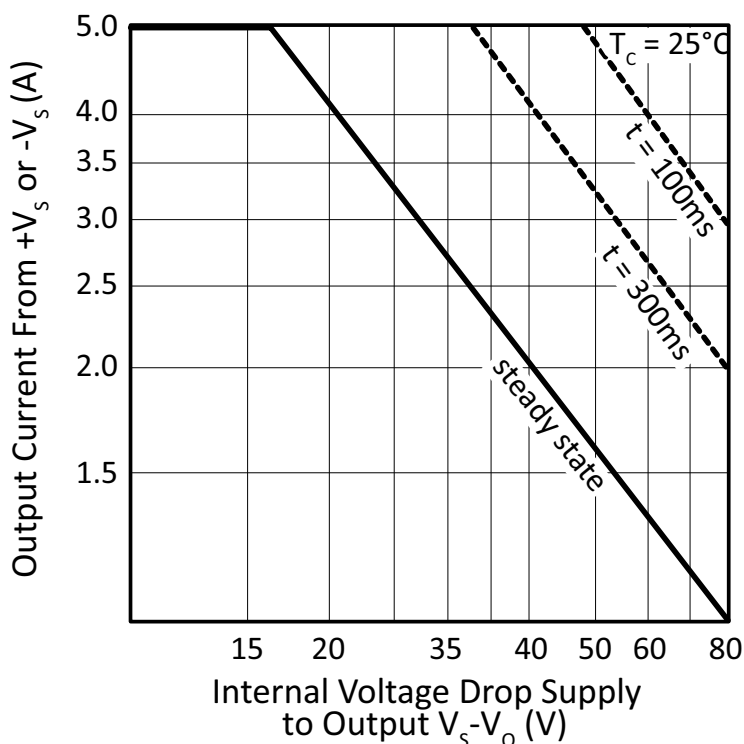
Figure 15: SOA
