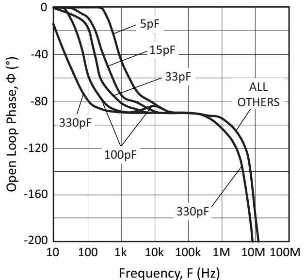
Figure 6: Phase Response
