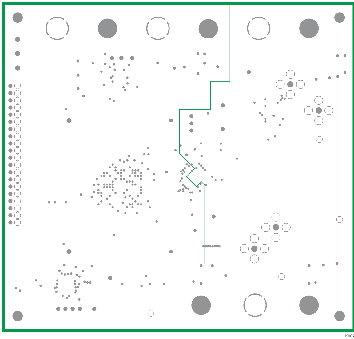
Figure 5. Layer 2, Ground Plane
