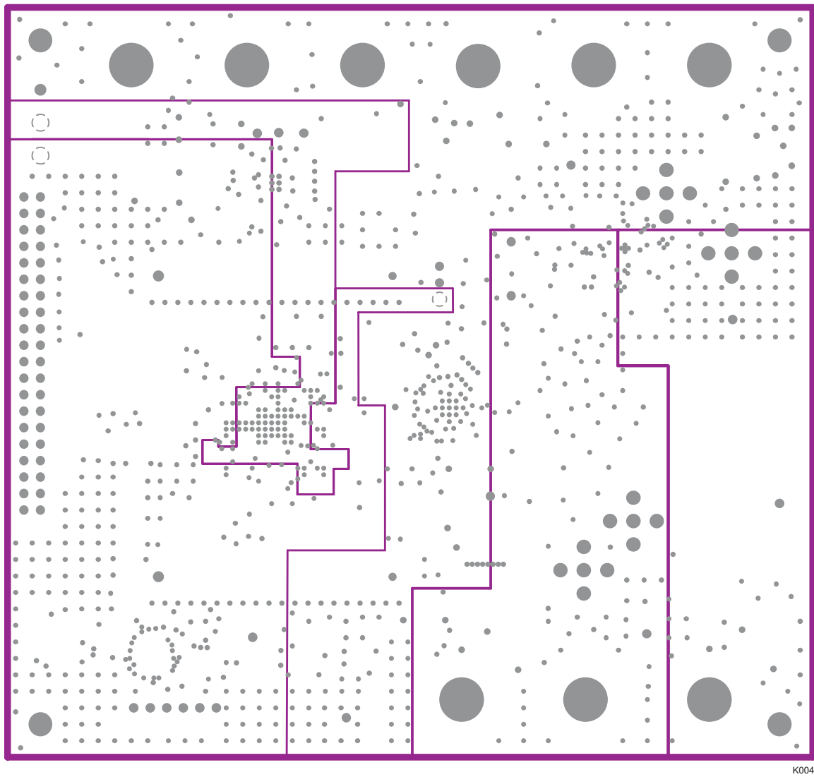
Figure 7. Layer 4, Power Plane #2
