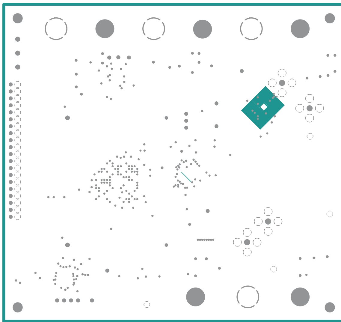
Figure 8. Layer 5, Ground Plane
