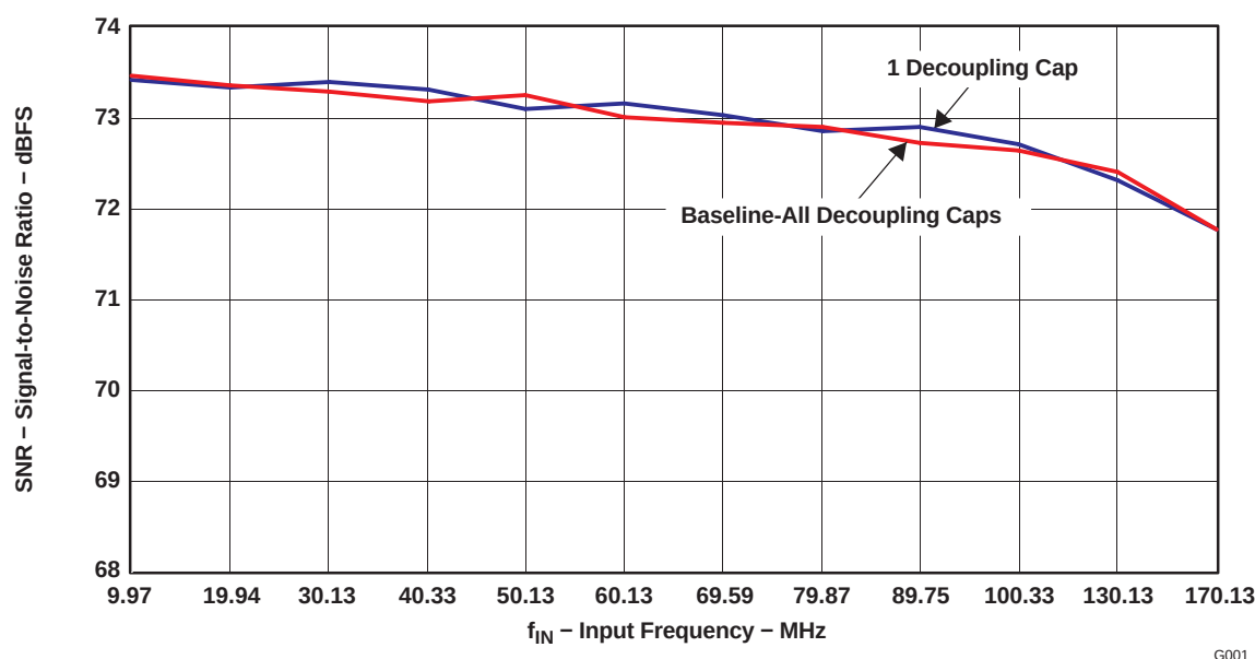
Figure 1. ADS5547 SNR Performance vs Decoupling
