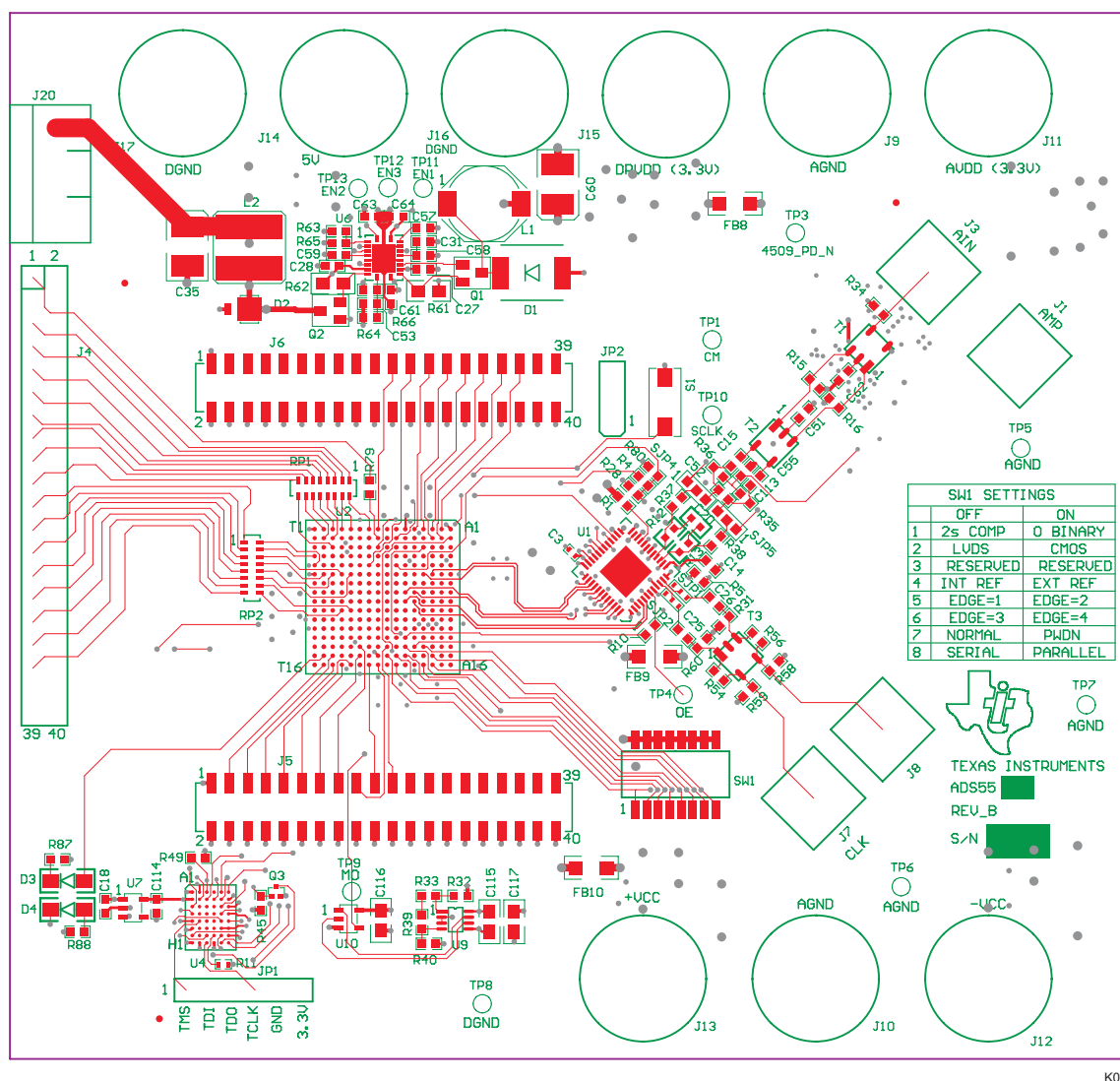
Figure 4. Top Layer
