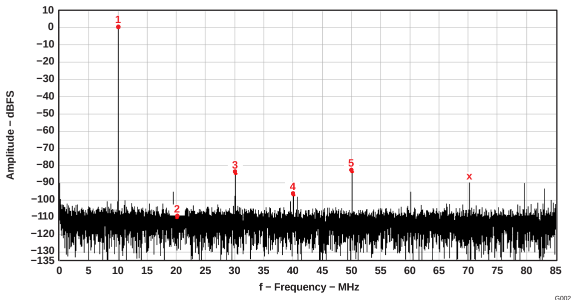
Figure 2. THS4509 + ADS5545 EVM Performance
