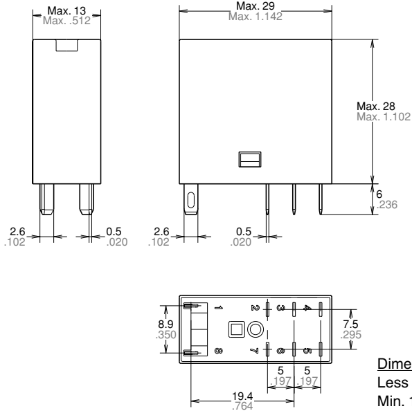
External dimensions
