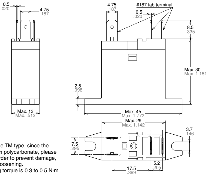
External dimensions
