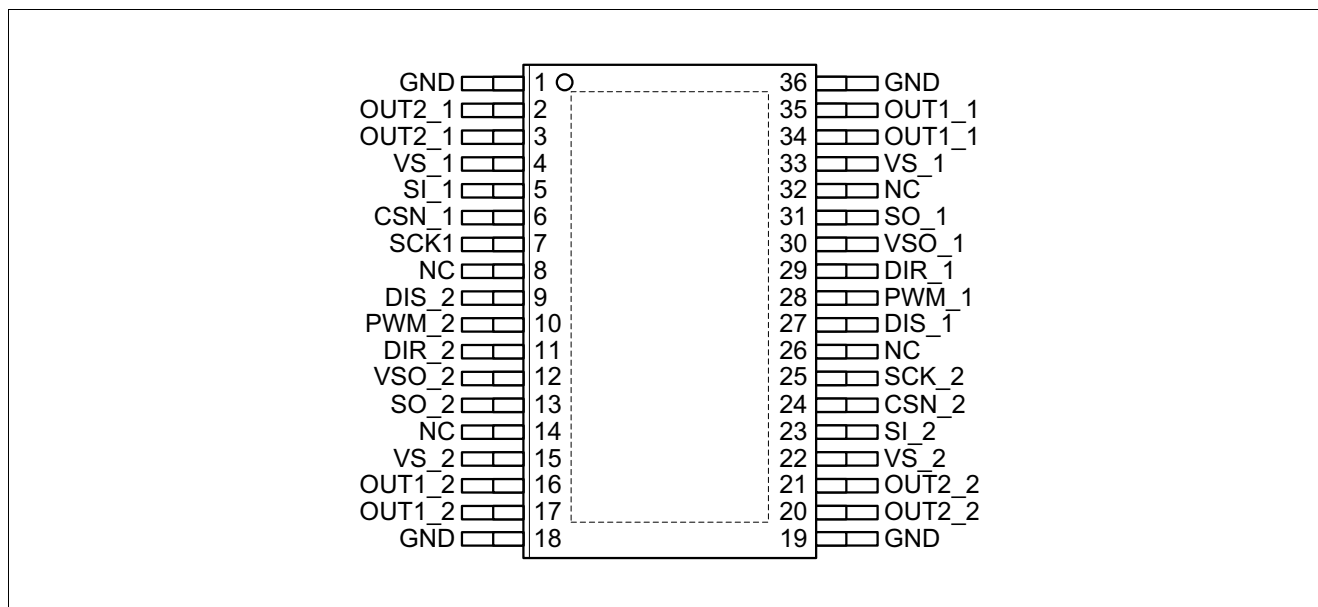
Figure 1 Pin Configuration IFX9202ED
