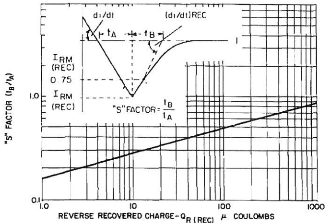
9. TYPICAL "S" FACTOR VERSUS RECOVERY CHARGE ( T_J = 175^\circ\text{C} )
