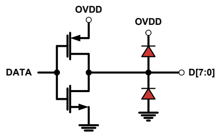
FIGURE 52. CMOS OUTPUTS
