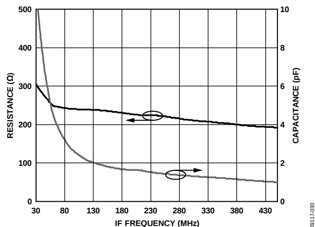
Figure 30. IF Differential Output Impedance (R Parallel C Equivalent)
