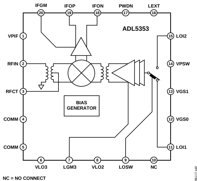
Figure 50. Simplified Schematic
