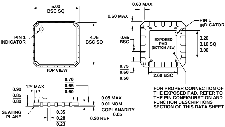
COMPLIANT TO JEDEC STANDARDS MO-220-VHHC Figure 57. 20-Lead Lead Frame Chip Scale Package [LFCSP_VQ] 5 mm x 5 mm Body, Very Thin Quad (CP-20-5) Dimensions shown in millimeters
