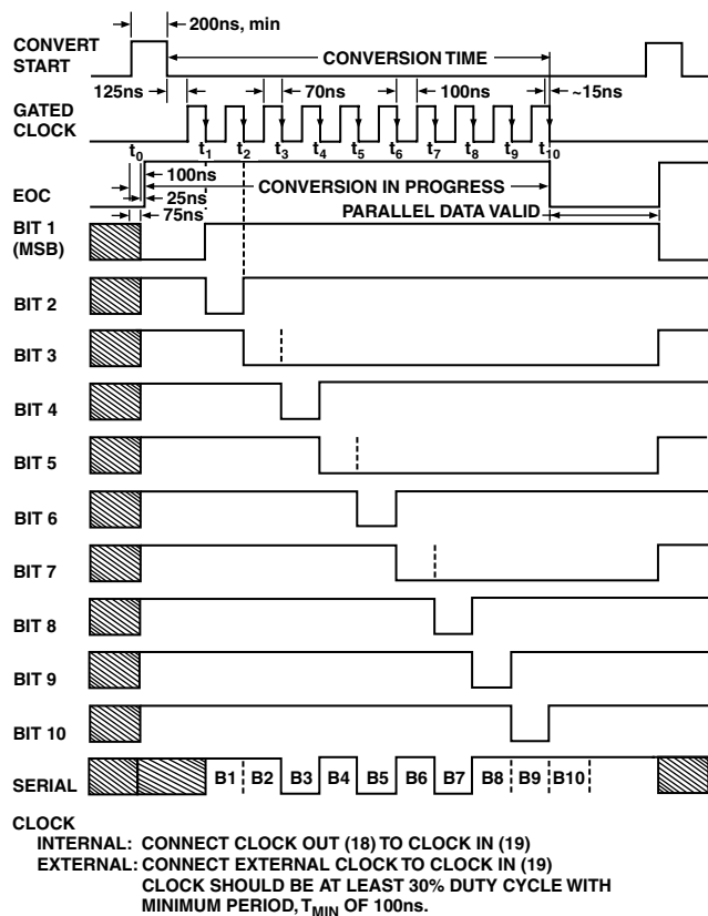
Figure 2b. AD579 Timing Diagram
