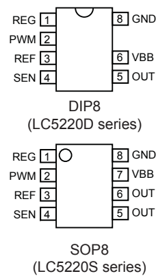
Pin-out Diagrams
