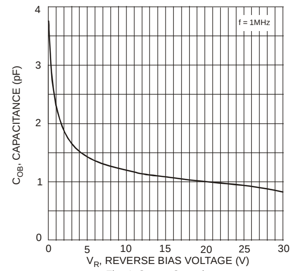
Fig. 4 Output Capacitance
