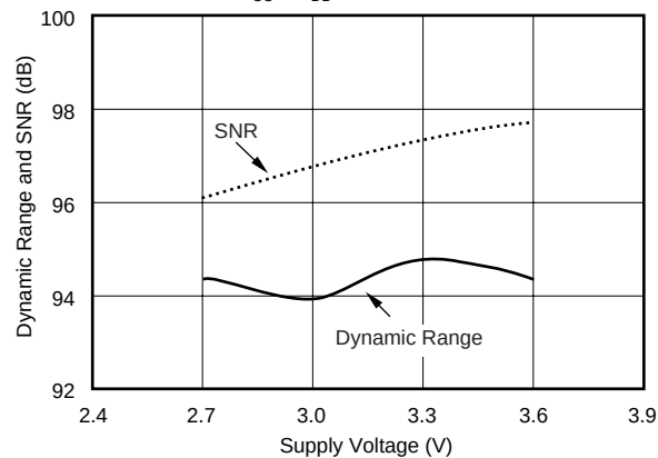
DYNAMIC RANGE AND SIGNAL-TO-NOISE RATIO vs SUPPLY VOLTAGE ( V_{CC} = V_{DD} = +2.7\text{V} to +3.6\text{V} )
