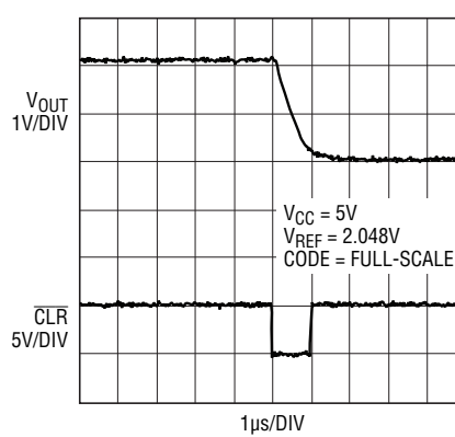
Hardware \overline{\text{CLR}} to Mid-Scale
