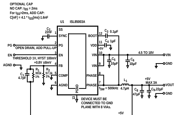
FIGURE 1B. ISL85003A V_{IN} RANGE FROM 4.5V TO 18V, V_{OUT} = 5V AND INTERNAL COMPENSATION WITH EXTERNAL SOFT-START
