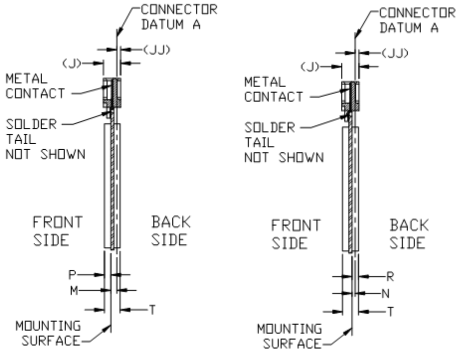
Figure 2: Connector location
