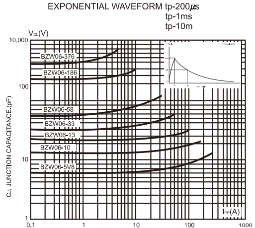
FIG.4-CLAMPING VOLTAGE VERSUS PEAK PULSE CURRENT.
