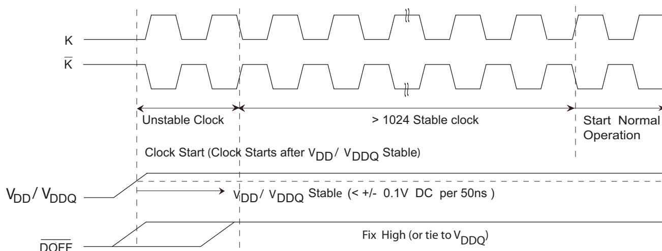
Figure 3. Power-up Waveforms
