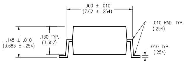
END VIEW
