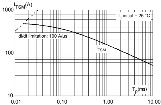
Figure 7. Non repetitive surge peak on-state current
