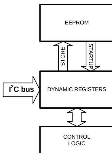
Figure 17. Register Structure
