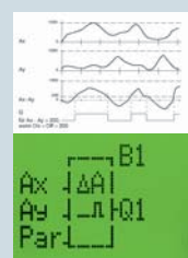
Analog comparator
