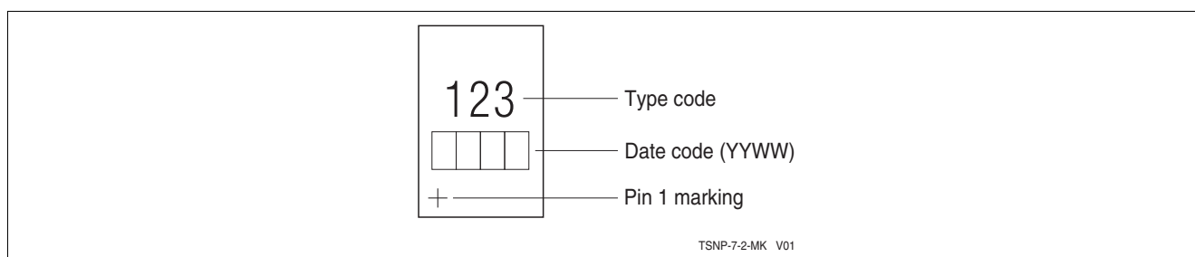
Figure 7 Marking Layout TSNP-7-2 (top view)
