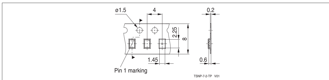
Figure 8 Tape & Reel Dimensions TSNP-7-2 (Ø reel 180, pieces/reel 6000)
