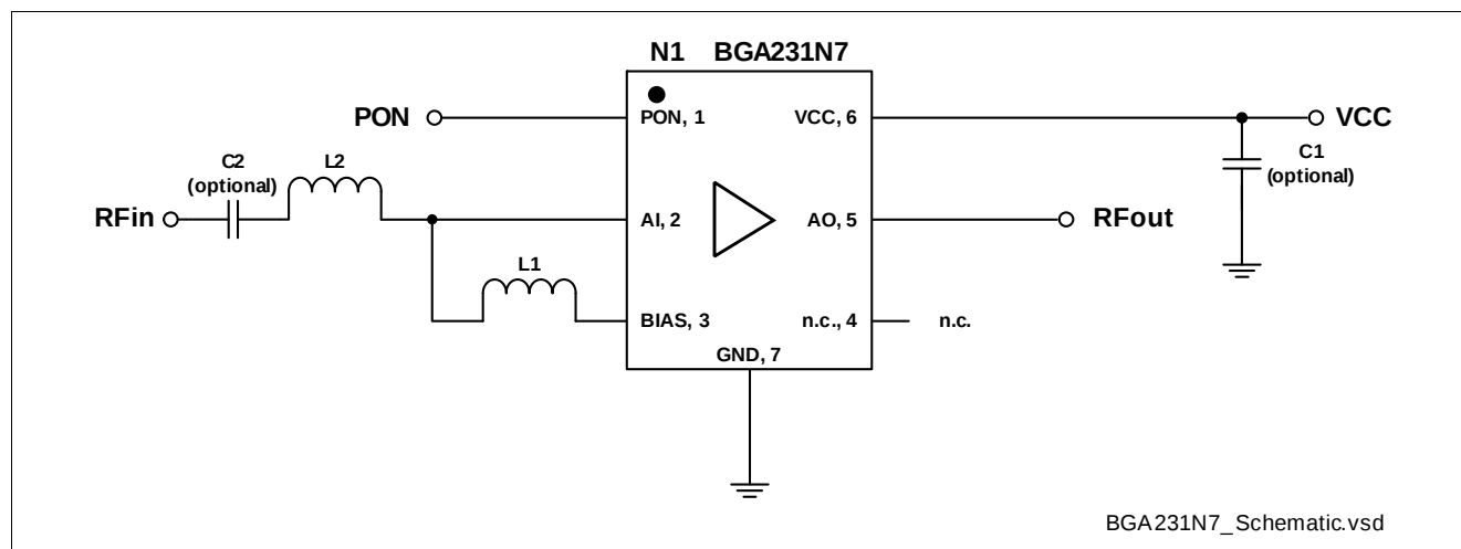
Figure 2 Application Schematic BGA231N7
