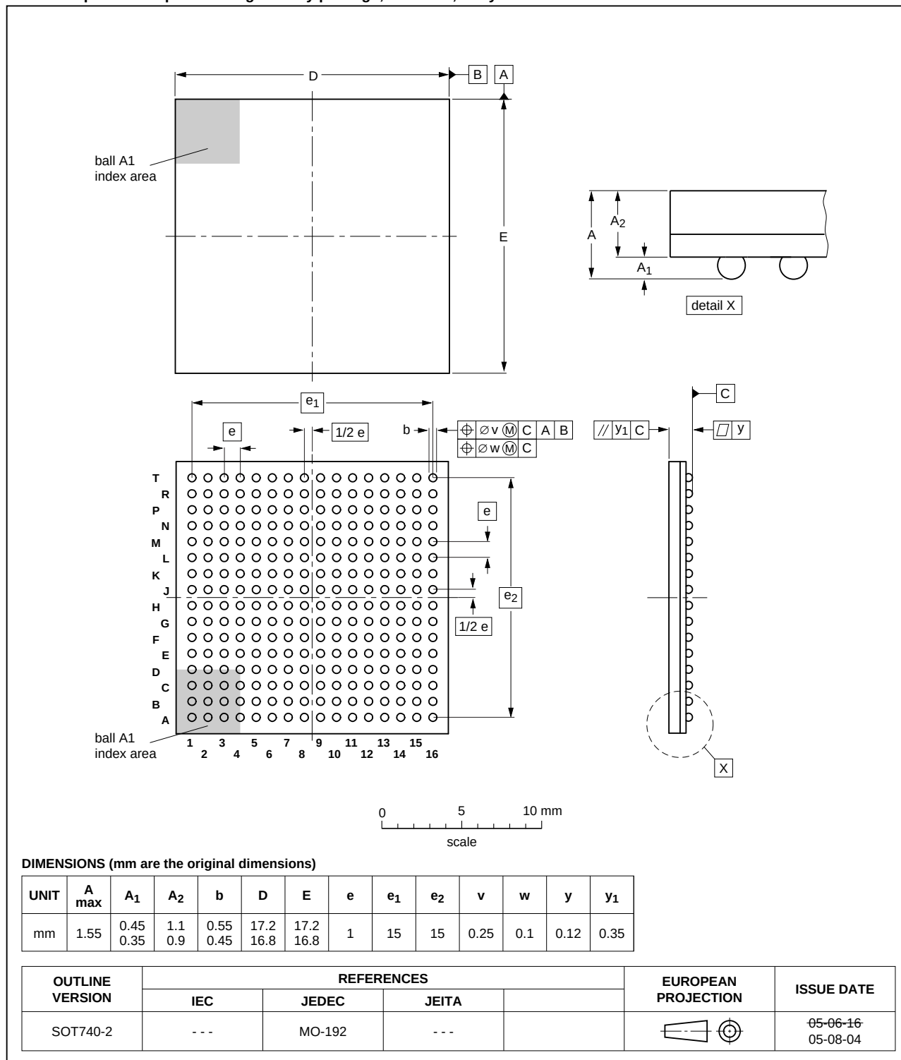
Fig 48. Package outline of the LPGA256 package
