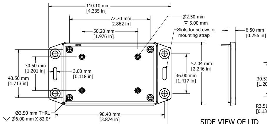
BOTTOM VIEW OF LID
