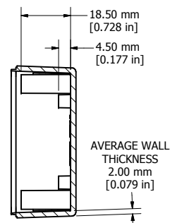
SECTION K-K
