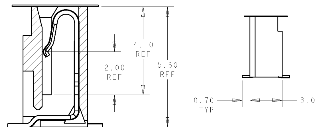
SECTION A-A (FOR EVEN POSITION CONTACTS) SCALE 10:1
