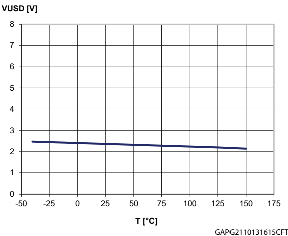
Figure 24. Undervoltage shutdown
