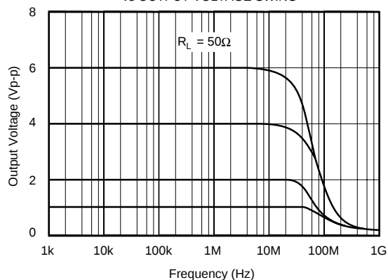
A_V = +10\text{V/V} CLOSED-LOOP BANDWIDTH vs OUTPUT VOLTAGE SWING
