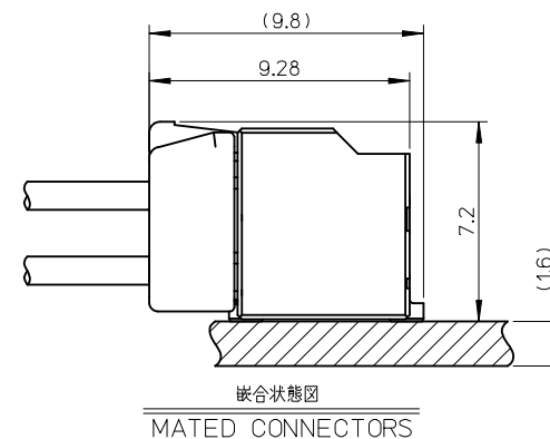
MATED CONNECTORS
