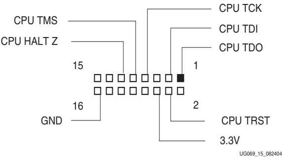
Figure 2-15: CPU Debug Connector Pinouts
