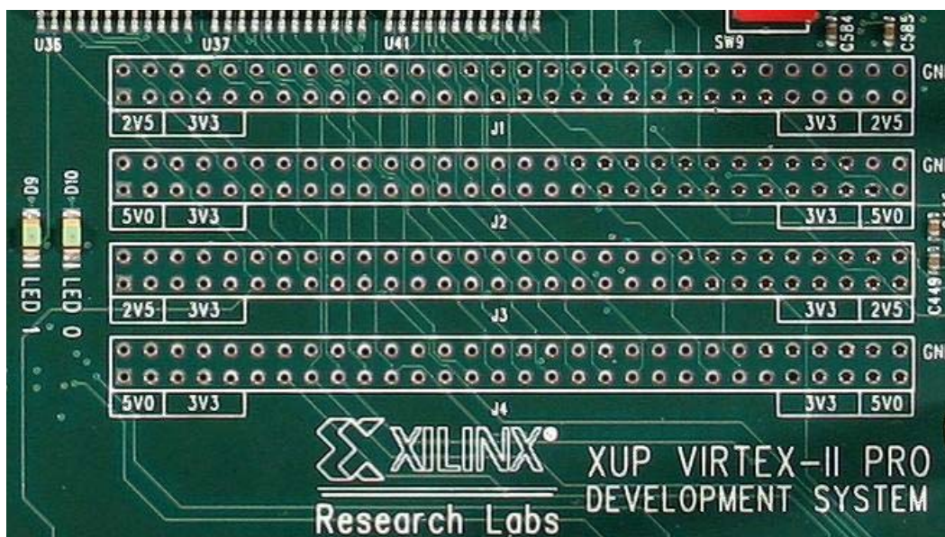
Figure 2-14: Expansion Headers
