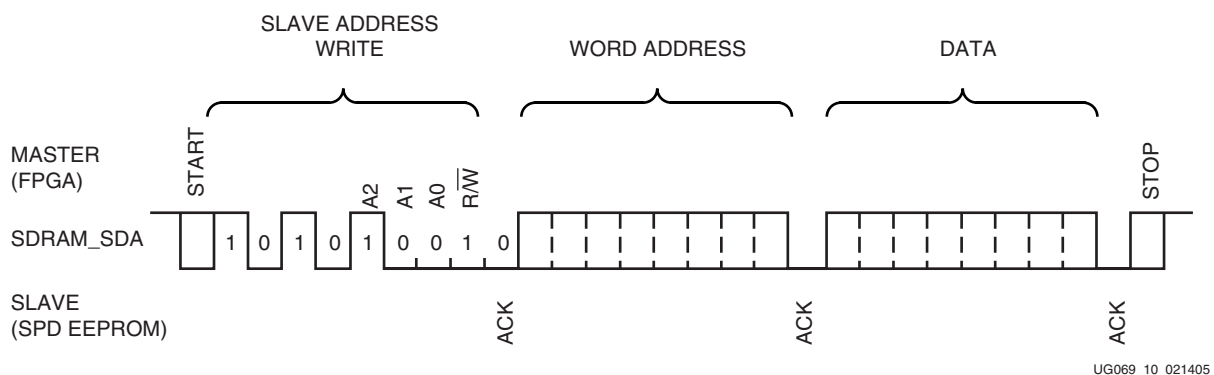
Figure 2-9: EEPROM Write
