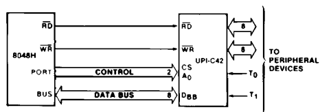
Figure 9. 8048H-UPI-C42 Interface
