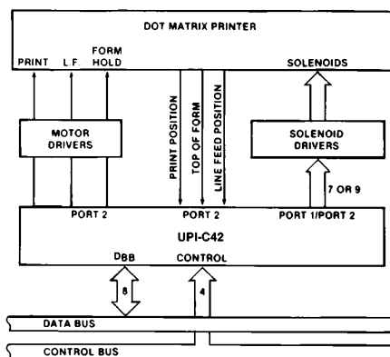
Figure 11. UPI-C42 80-Column Matrix Printer Interface
