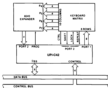
Figure 10. UPI-C42-8243 Keyboard Scanner
