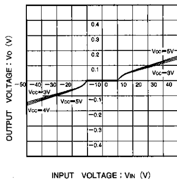
Fig. 7 Dead zone I/O characteristics
