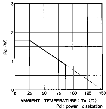
Fig. 4 When mounted to a 50 × 50 × 1.0 (mm) paper phenol board
