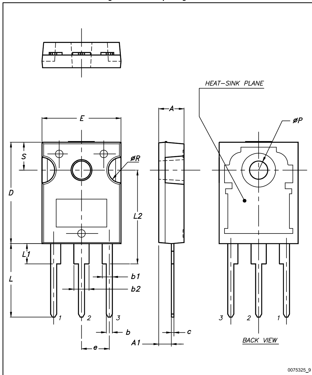
Figure 26: TO-247 package outline
