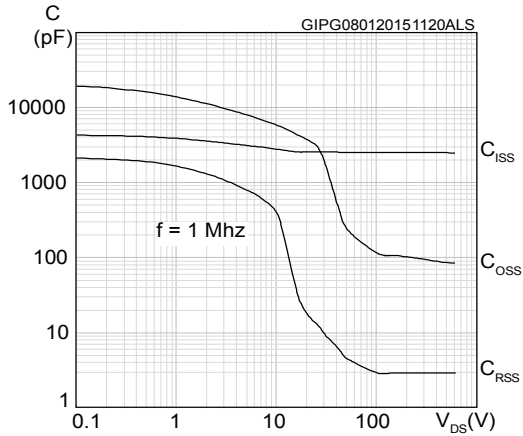
Figure 10: Capacitance variations
