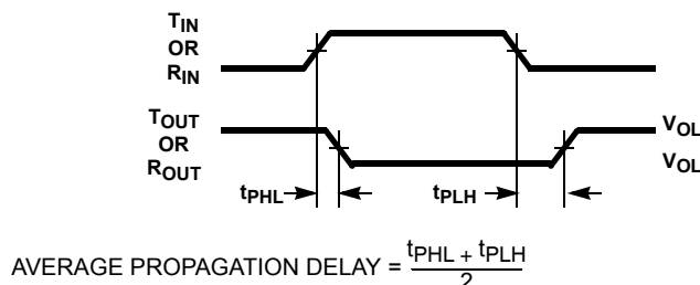
FIGURE 4. PROPAGATION DELAY DEFINITION
