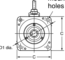
Four, Z-dia. mounting holes
