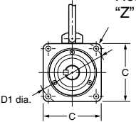
Hole with "Z" mark
