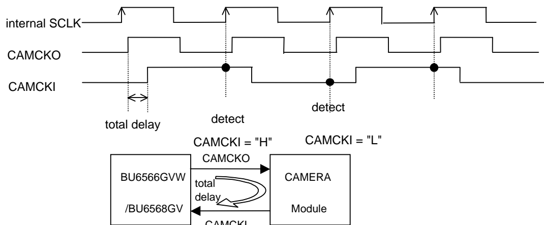
Figure .2.1-1 Relation between system clock and camera clock
