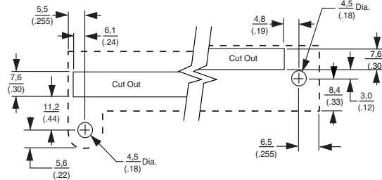
RIGHT ANGLE VERTICAL MOUNTING PANEL LAYOUT
